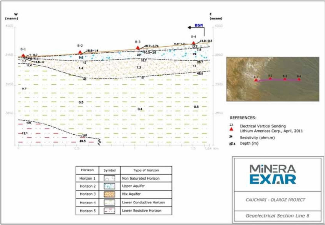
Figure 9.15 VES Survey Interpretation Along Line 8
