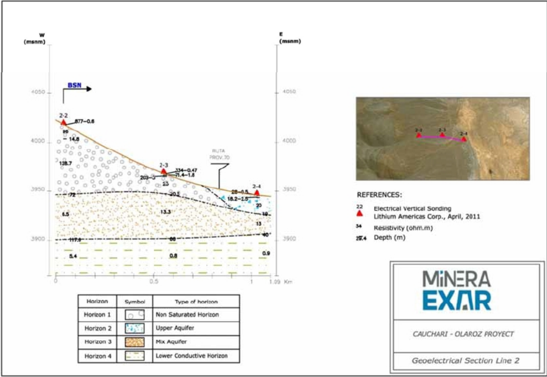
Figure 9.14 VES Survey Interpretation Along Line 2
