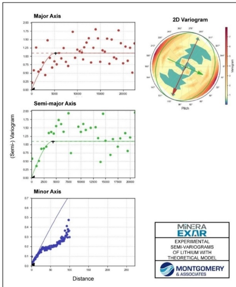
Figure 14.18 Experimental Semi-Variograms of Lithium with Theoretical Model
