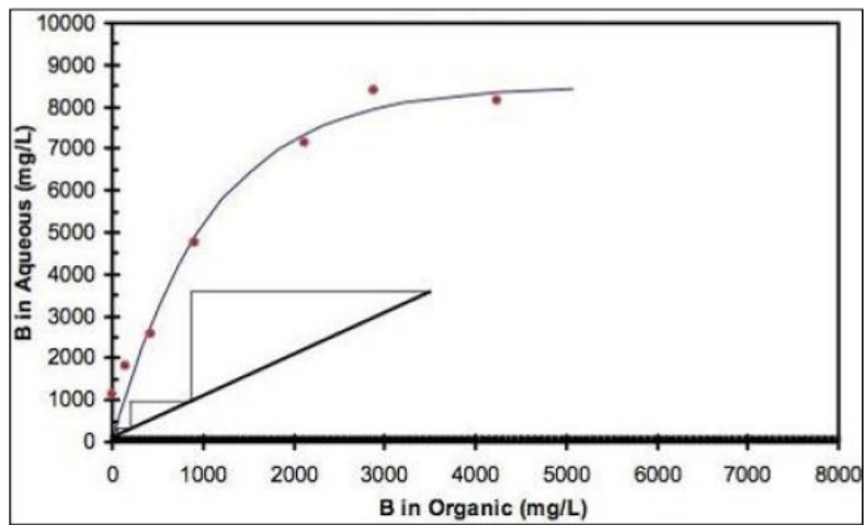
Figure 13.9 Re-extraction Isotherm at 20 °C Using Mixed Extractants
