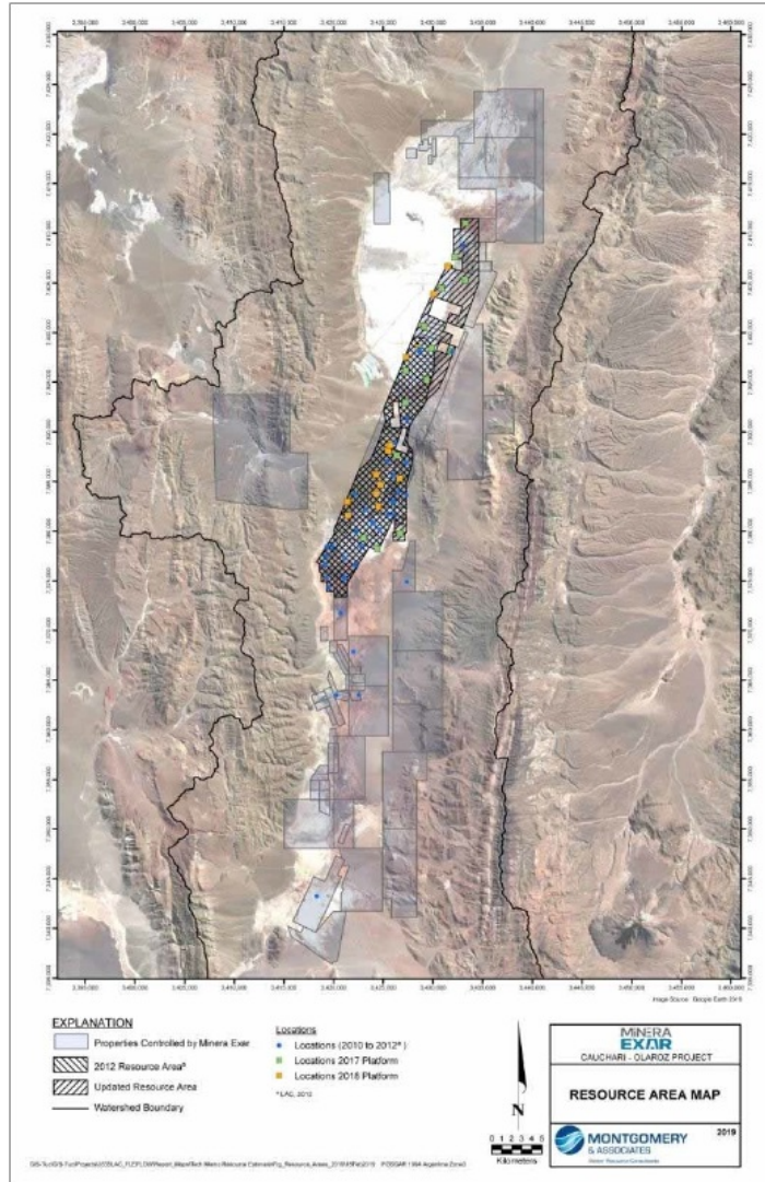
Figure 14.5 Location Map Showing Resource Evaluation Areas - 2012 Mineral Resource Estimate and Updated Mineral Resource Estimate
