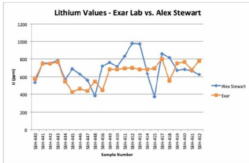
Figure 12.1 Due Diligence Sample Results for Lithium: February 2019
