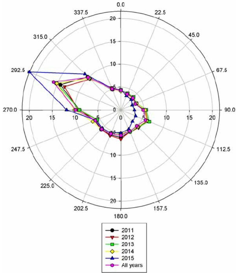
Figure 5.8 Prevailing Wind Directions, Vaisala Station, Cauchari, 2011-2015
