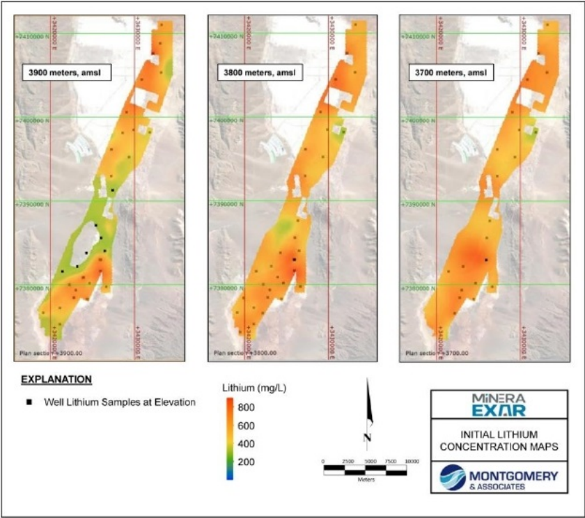
Figure 14.19 Representative Elevation Maps of Initial Lithium Concentrations for Updated Mineral Resource Estimate
