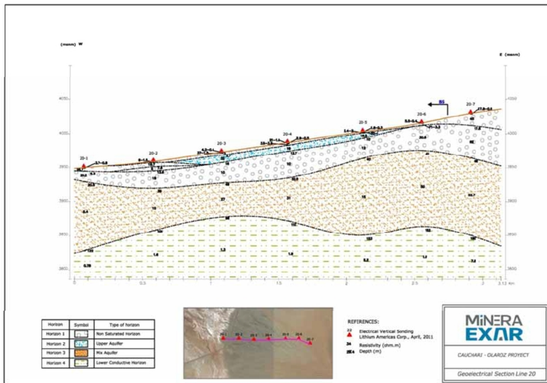
Figure 9.16 VES Survey Interpretation Along Line 20
