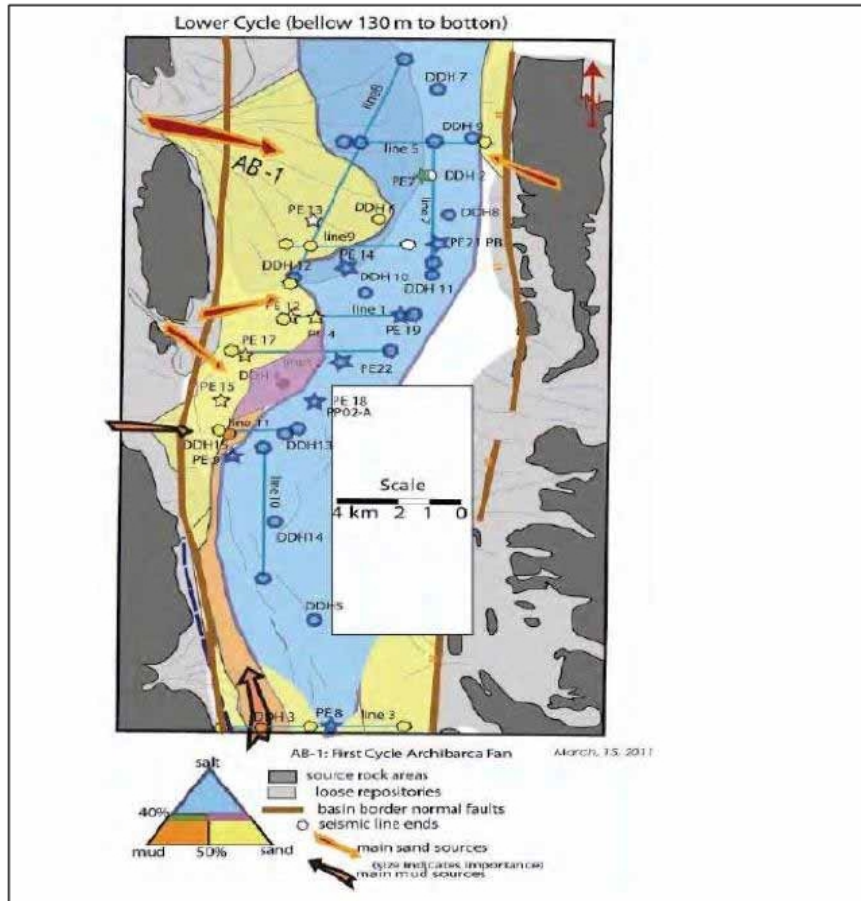
Figure 7.4 Facies Map of the Lower Salt Cycle showing Line 1 Crossing a Thick Salt Succession
