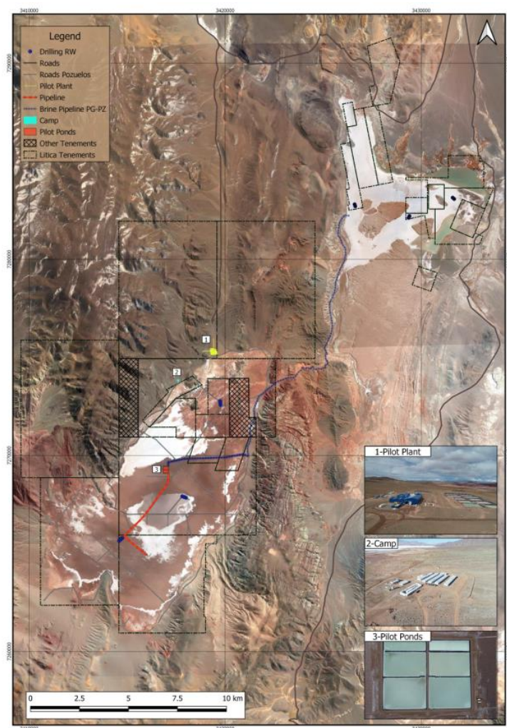
Figure 9: Main On-site Facilities and Areas (Source: Ganfeng, 2024)
