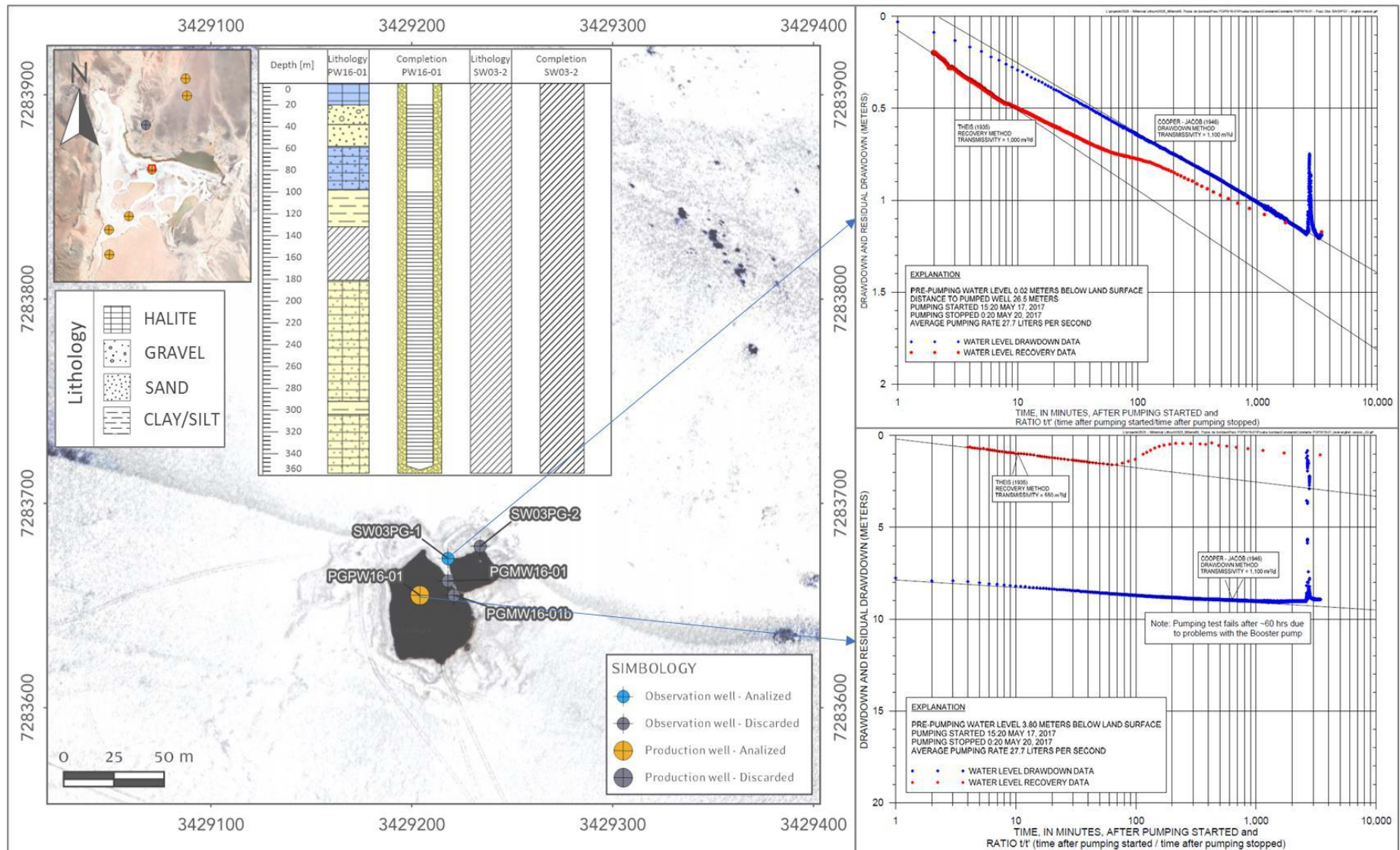
Figure 11: Location, setup and results of pumping test well PGPW16-01 (2017)
