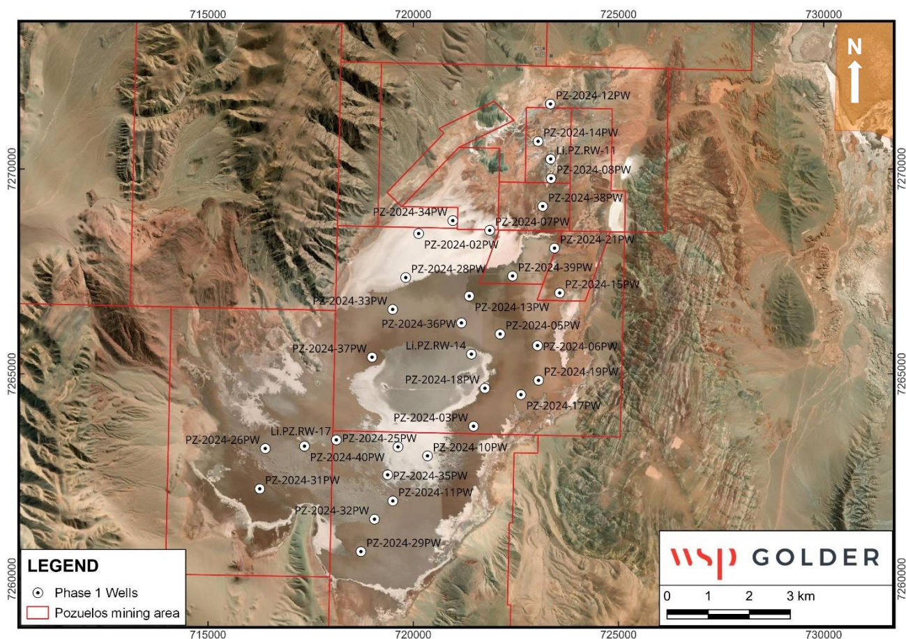
Figure 146: Production Wells for Phase 1
