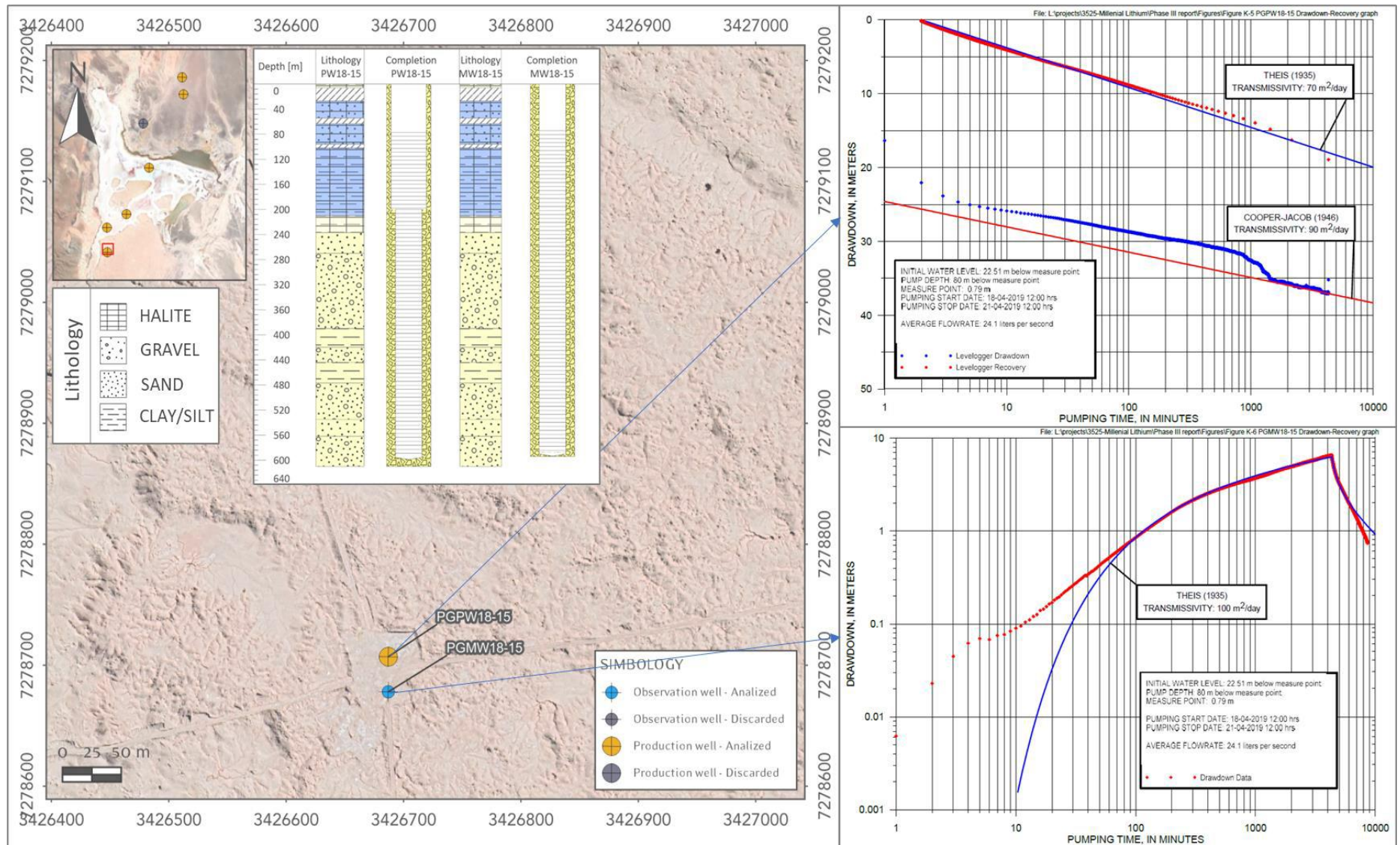
Figure 13: Location, setup and results of pumping test well PGPW18-15
