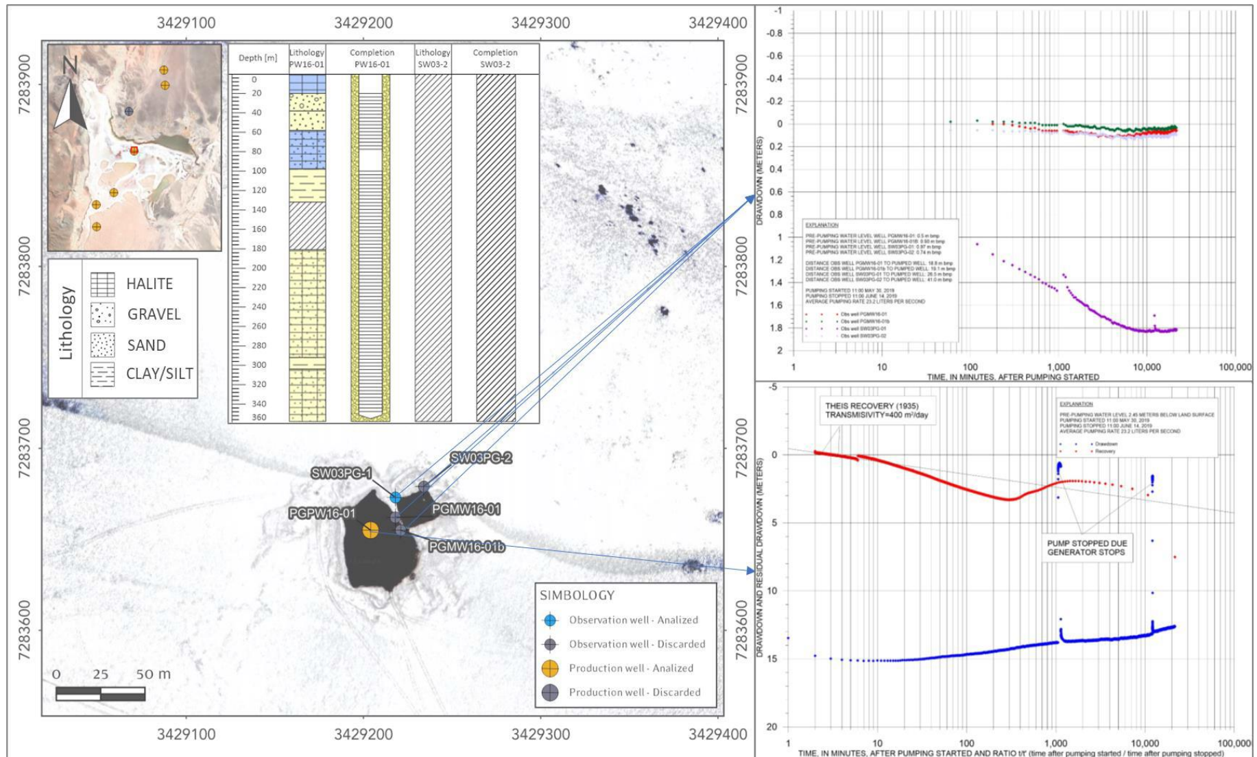
Figure 15: Location, setup and results of pumping test well PGPW16-01 (2019)
