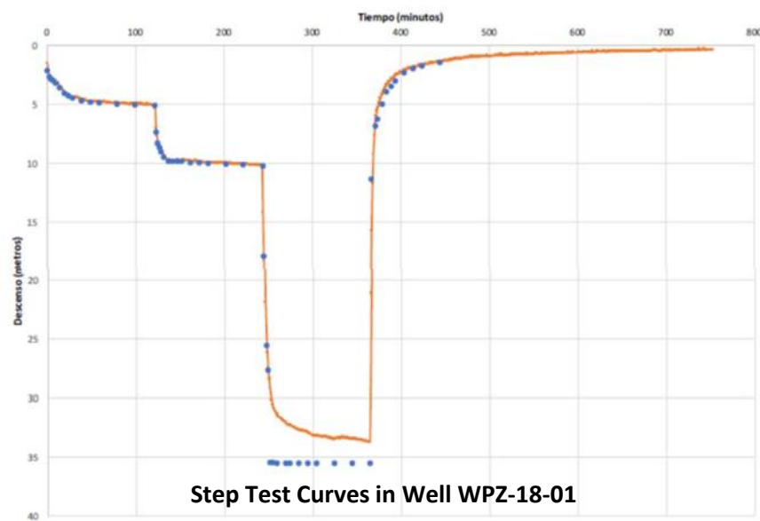
Figure 6: Step Test and Constant Rate Test Curves, Brine Assays and Hydraulic parameters in Well WPZ-18- 01(2018)
