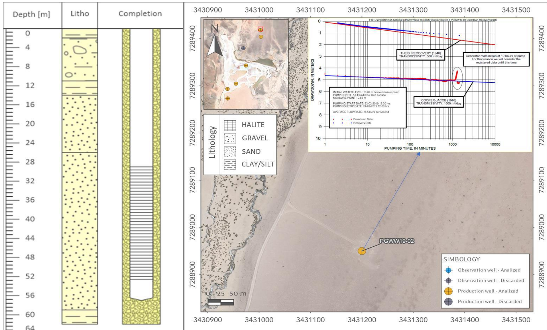
Figure 16: Location, setup and results of pumping test well PGPW19-02
