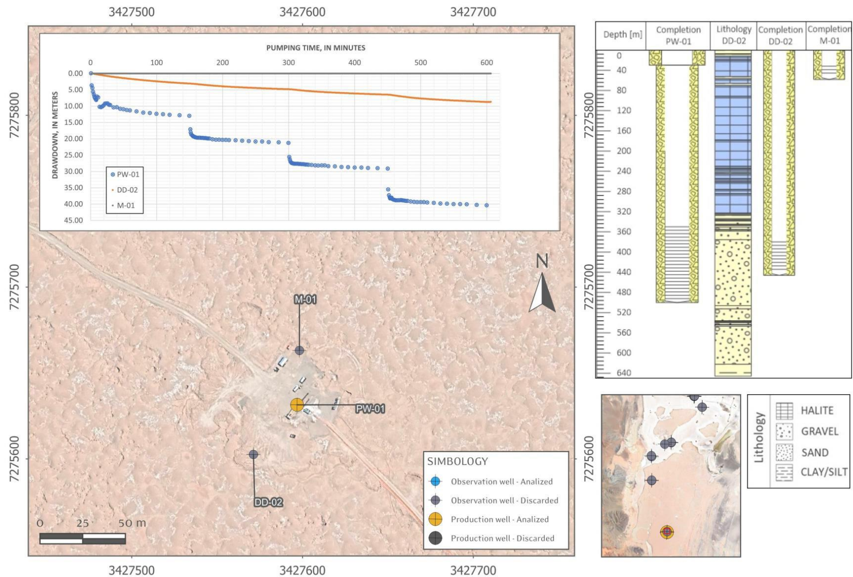
Figure 18: Location, setup and results of pumping test well PW-01
