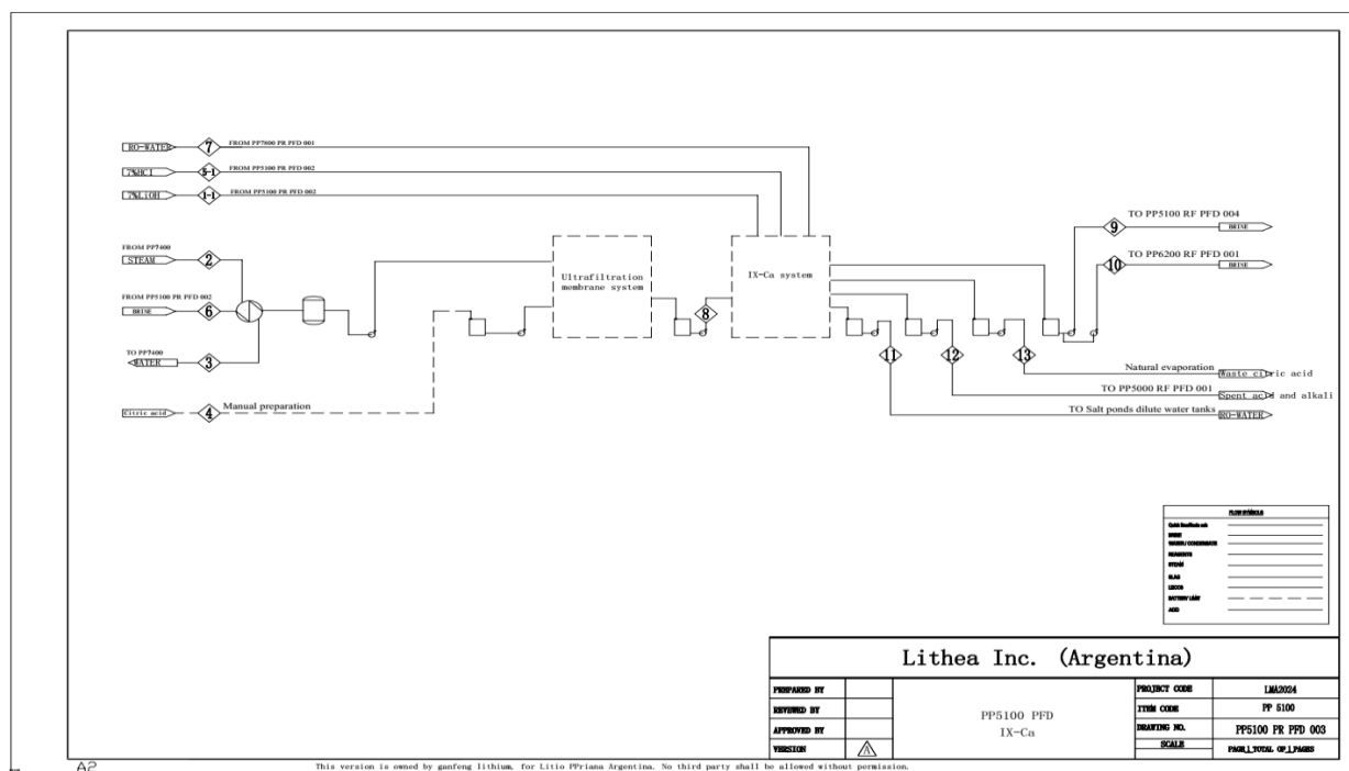
Figure 166: Flowsheet for Ca Removal Process (Source: Ganfeng, 2024)
