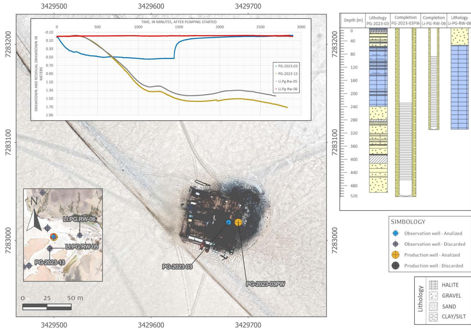
Figure 19: Location, setup and results of pumping test well PG-2023-03PW
