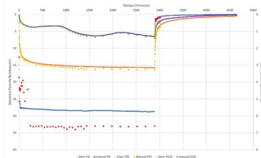
Figure 4: Step Test and Constant Rate Test Curves, Brine Assays and Hydraulic parameters in Well SP-2017-2W (2018)
