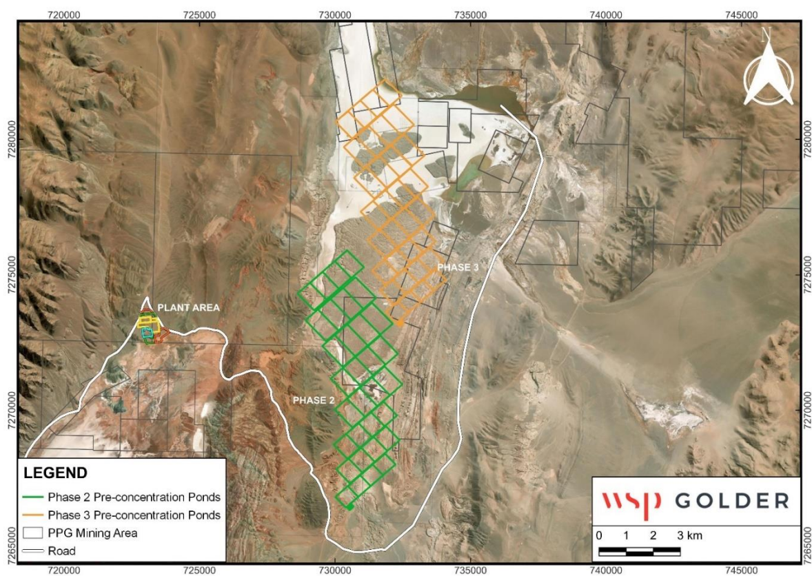
Figure 153: Phase 2 and 3 Ponds Layouts
