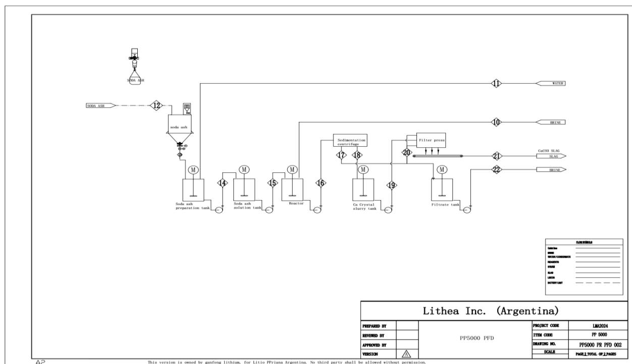
Figure 163: Flowsheet for Ca Removal Process (Source: Ganfeng, 2024)
