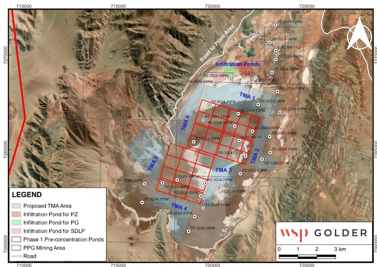
Figure 154: Proposed TMA and Infiltration Ponds for Phase 1
