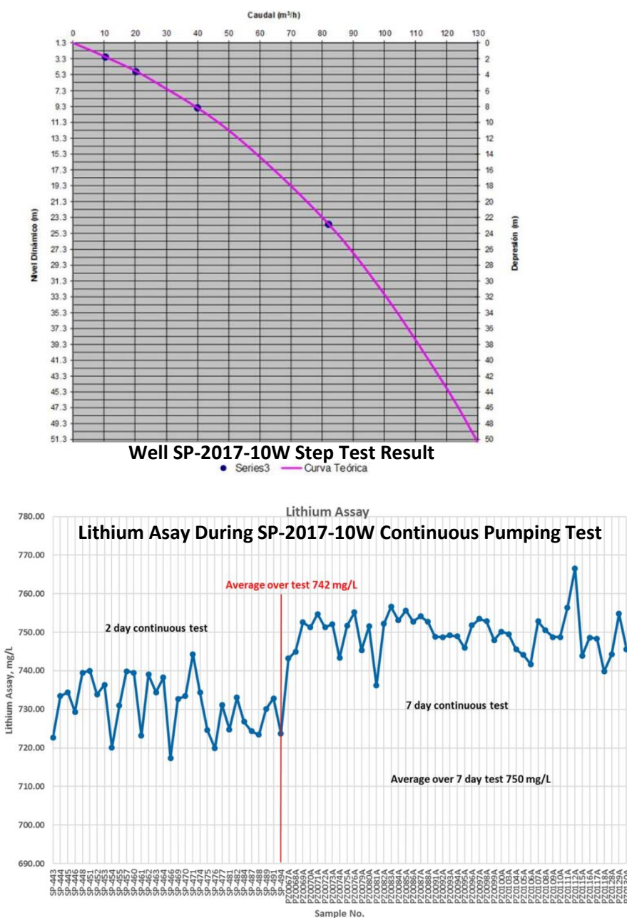
Figure 2: Step Test and Constant Rate Test Curves, Brine Assays and Hydraulic parameters in Well SP-2017-10W (2018)
