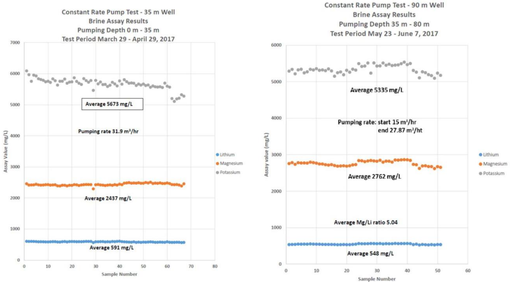
Figure 1: 2017 Constant Rate Pumping Test Brine Assays in Well PW1-35 (left) and Well P2-90 (right)
