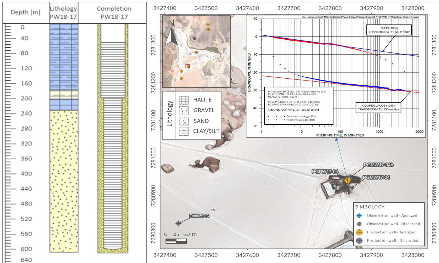
Figure 14: Location, setup and results of pumping test well PGPW18-17
