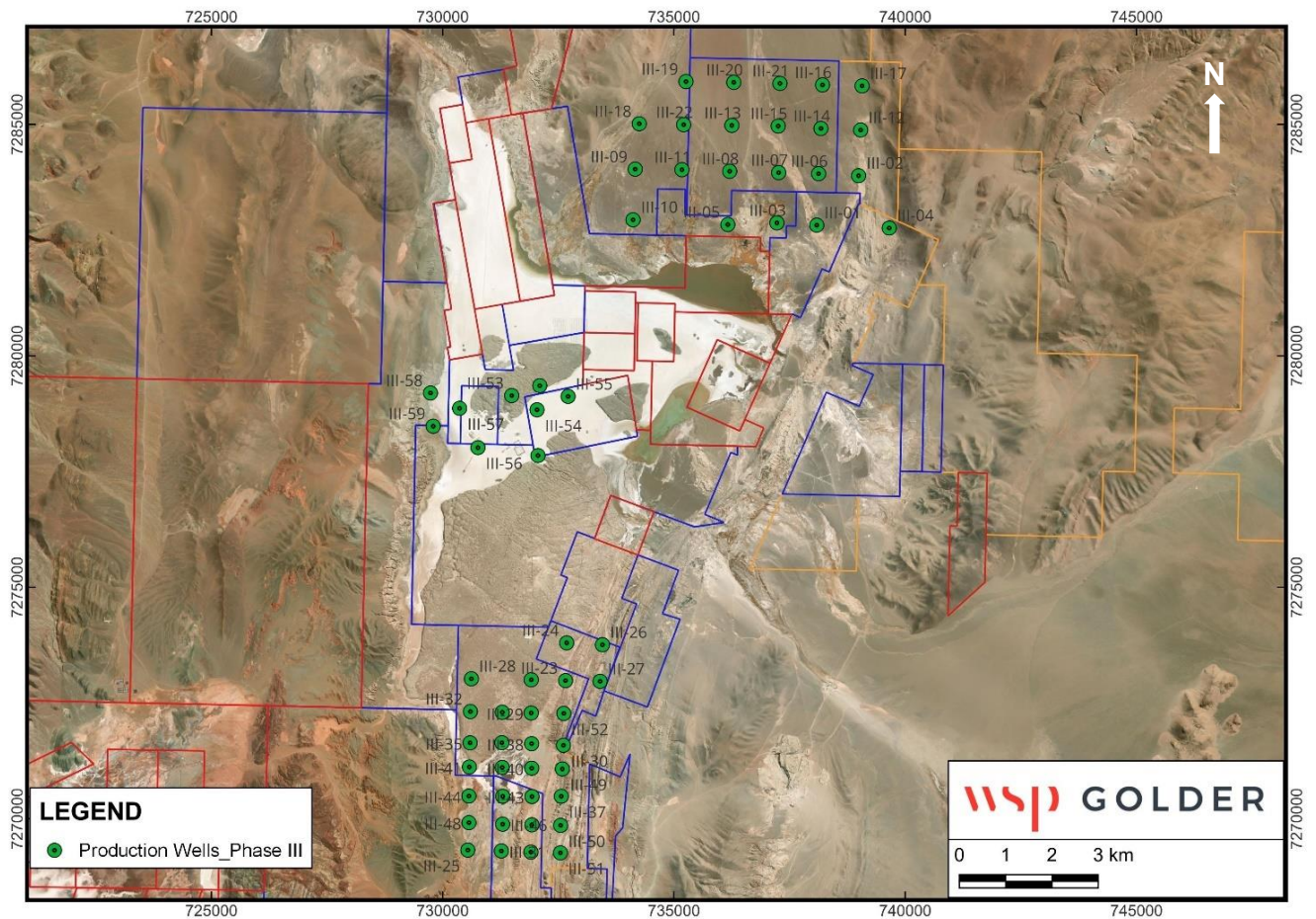
Figure 148: Proposed Production Wells for Phase 3
