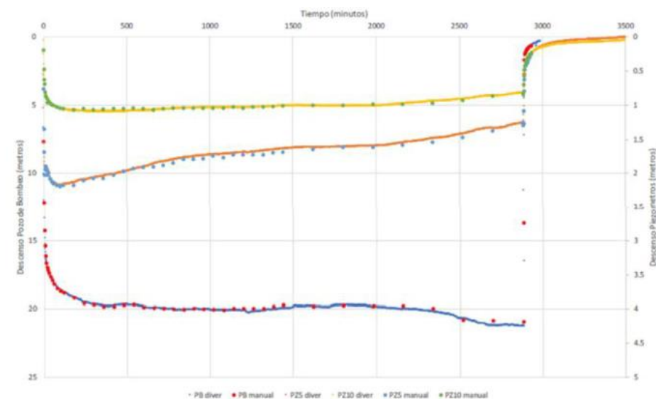
Figure 5: Step Test and Constant Rate Test Curves, Brine Assays and Hydraulic parameters in Well SP-2017-14W (2018)
