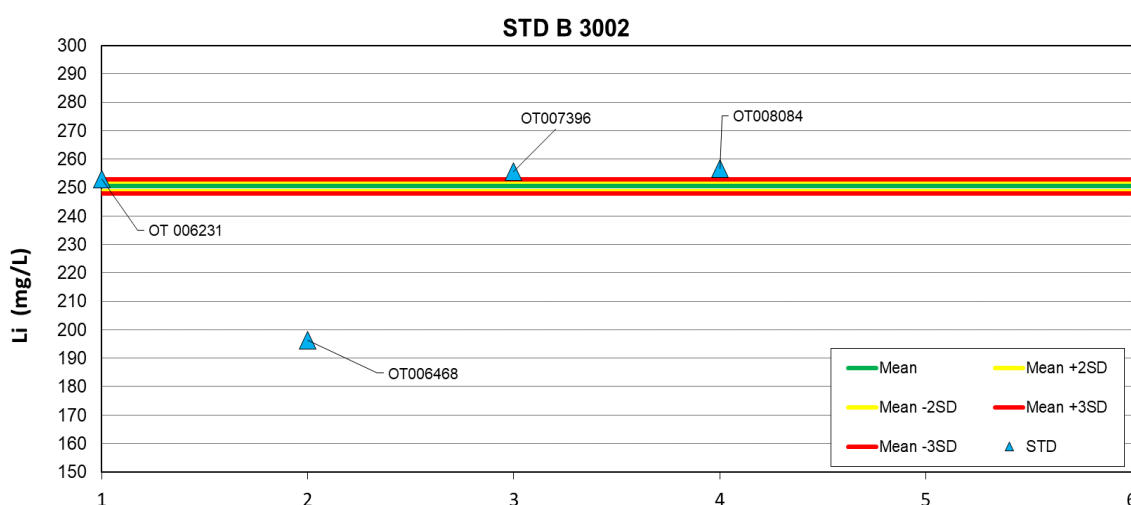
Figure 70: Performance of the Reference Sample TDS B 3002 (Source: WSP Golder, Jan 2025)
