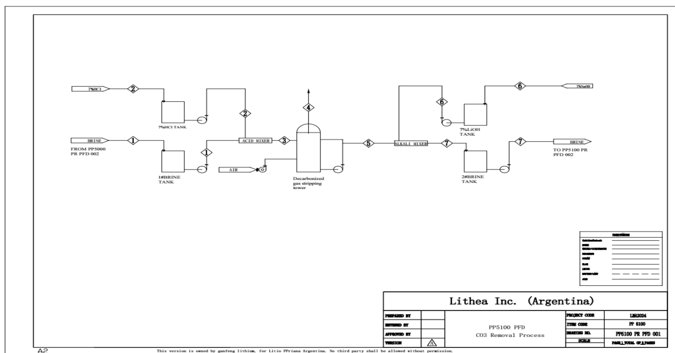
Figure 164: Flowsheet for Carbonate Removal Process (Source: Ganfeng, 2024)
