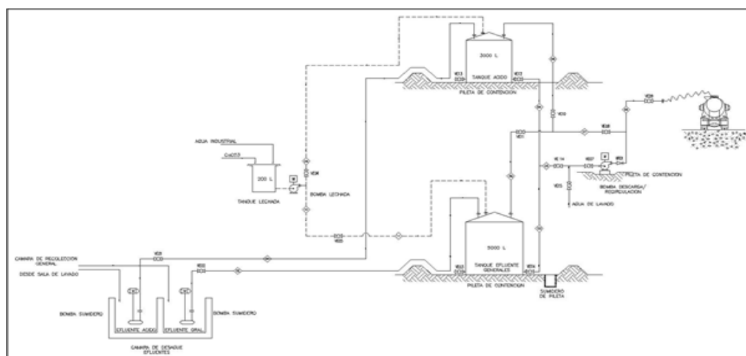
Figure 211: Acid Effluent Neutralization System (Source: Ganfeng, 2024)
