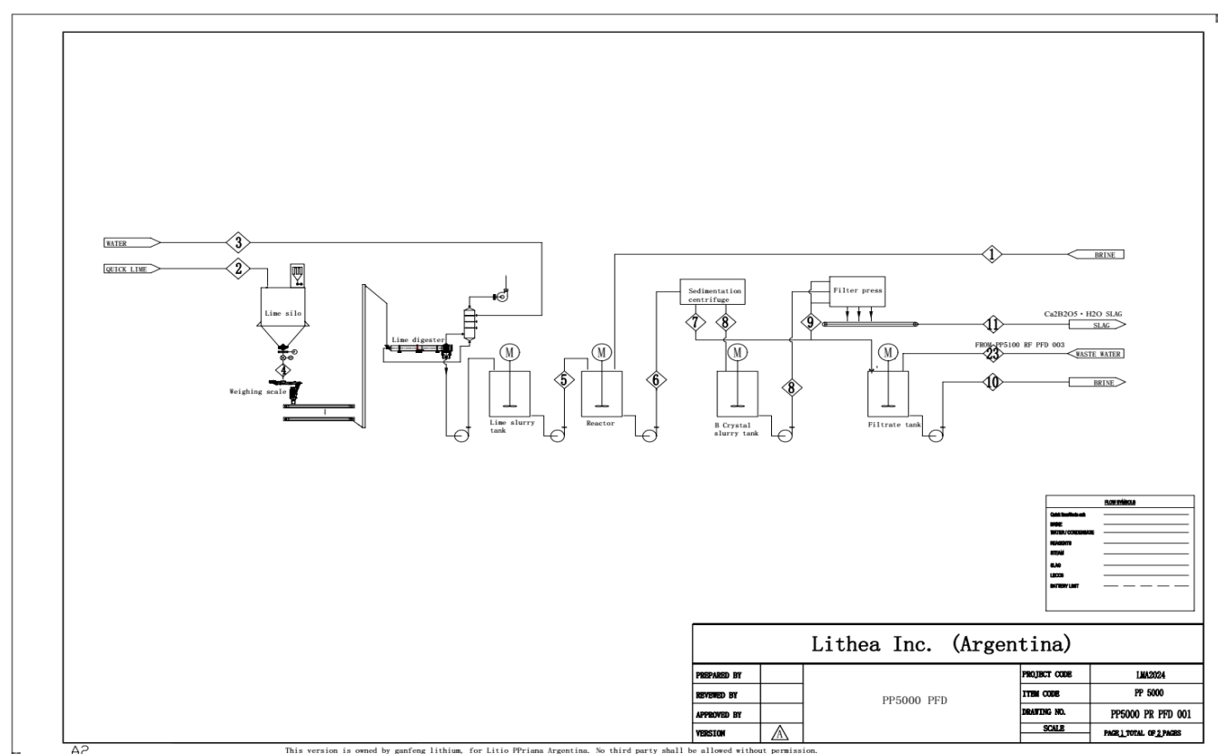
Figure 161: Process Flow Diagram of Boron Removal in Primary Purification Plant (Source: Gangfeng, 2024)
