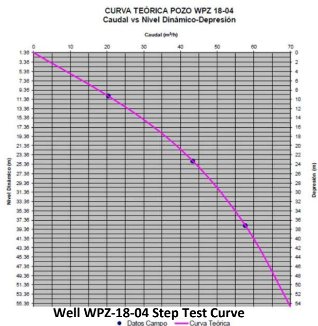
Figure 3: Step Test Curve, Brine Assays and Hydraulic parameters in Well WPZ-18-04 (2018)
