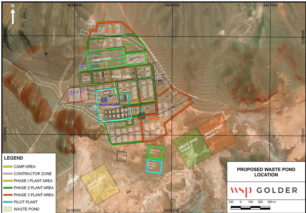
Figure 162: Location of the Plant's Solid Waste Deposit (Source: WSP Golder, Jan 2025)
