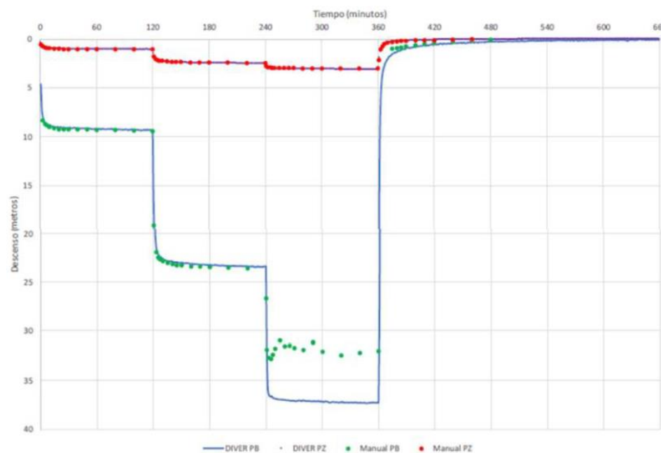
Figure 3: Step Test Curve, Brine Assays and Hydraulic parameters in Well WPZ-18-04 (2018)
