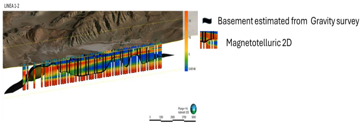
Figure 35: Magnetotellurics and Highs and Downs of the Gravity Line 1-2 (Proingeo 2021)
