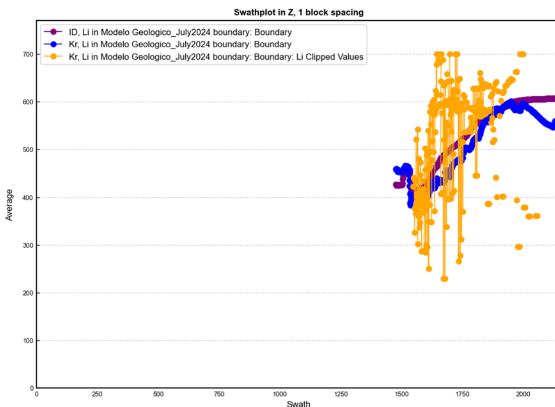
Figure 104: Swat Plot Showing the Concentrations of Lithium from the Samples, Kriging and Inverse Distance Estimator (Source: WSP Golder, Jan 2025)
