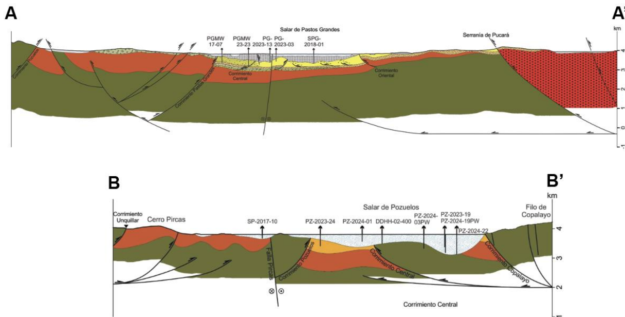
Figure 12: Representative Geological and Structural Cross Sections of Pastos Grandes (upper) and Pozuelos (lower). Note: cross sections are not the same scale.
