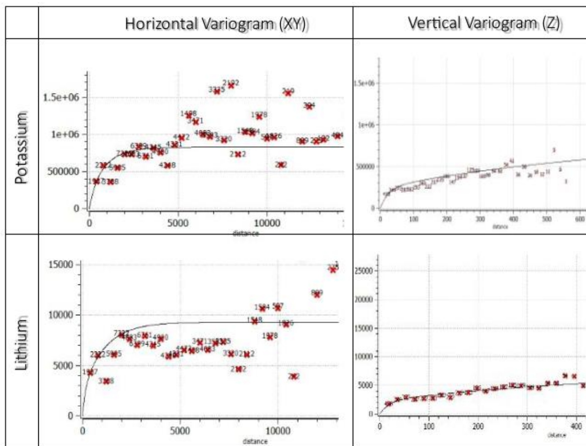
Figure 115: Experimental Variogram and Variogram Model for Potassium and Lithium in Region I (Source: AW, Dec 2024)
