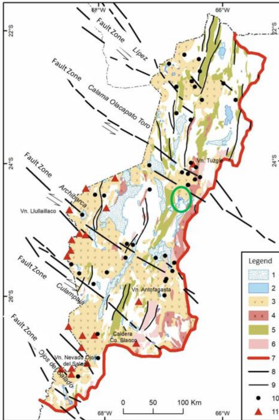
Figure 10: Geological Map of the Puna (Modified from Viramonte and Petrinovic 1990; Lizuain Fuentes et al. 2018)
