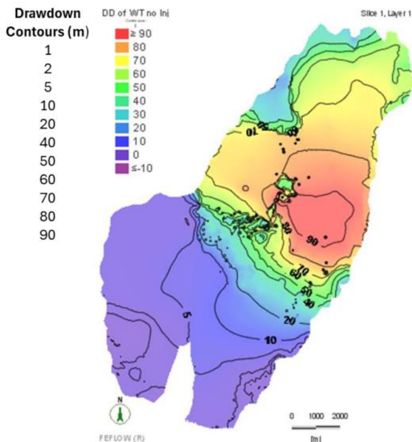
Figure 126: Simulated Drawdown without Infiltration (Source: AW, September 2024)
