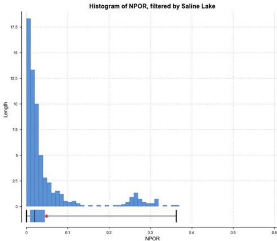
Figure 101: Histograms for Porosities of the Saline Lake (Source: WSP, Jan 2025)
