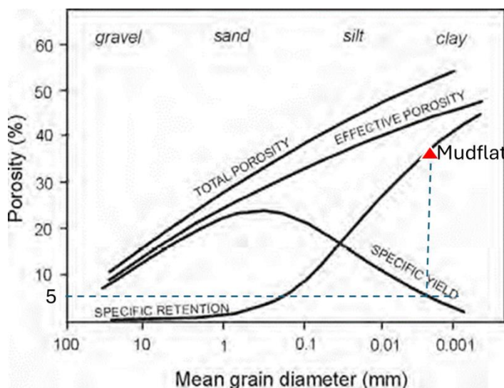
Figure 68: Porosity Relationships for Unconsolidated Material (Source: Johnson 1967)
