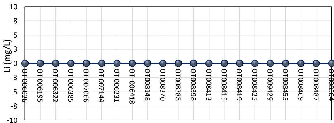
Figure 74: Blanks Performance (Source: WSP Golder, Jan 2025)
