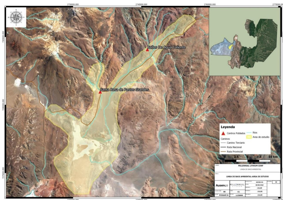
Figure 197: Environmental Baseline Study Area (Source: Ausenco, 2018)
