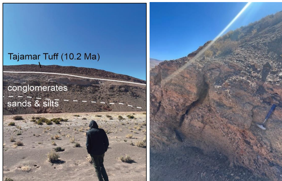
Figure 17: Verde Conglomerate Overlying Sands and Silts of the Pozuelos Formation and Underlying Tajamar Tuff (left) and a Close-up Photograph of the Unit in Outcrop (right) (Source: LAR, 2025)
