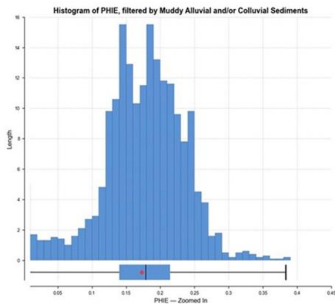
Figure 100: Histograms of the Sy (PHIEE) for the Muddy Alluvial and Colluvial Sediments (Source: WSP Golder, Jan 2025)
