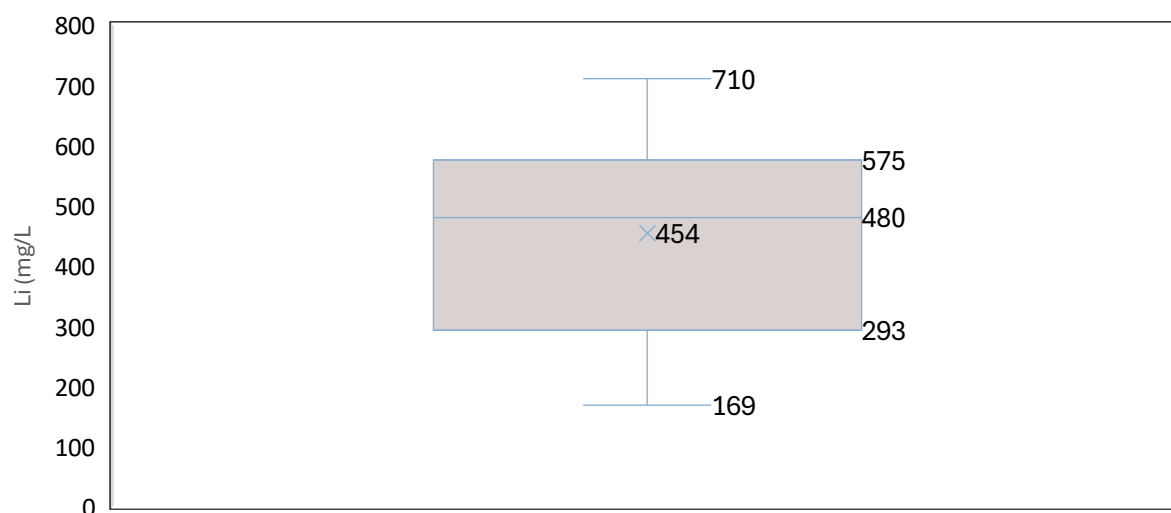
Figure 61: Lithium Concentration in the Central Zone from Pozuelos (Source: WSP Golder, Jan 2025)
