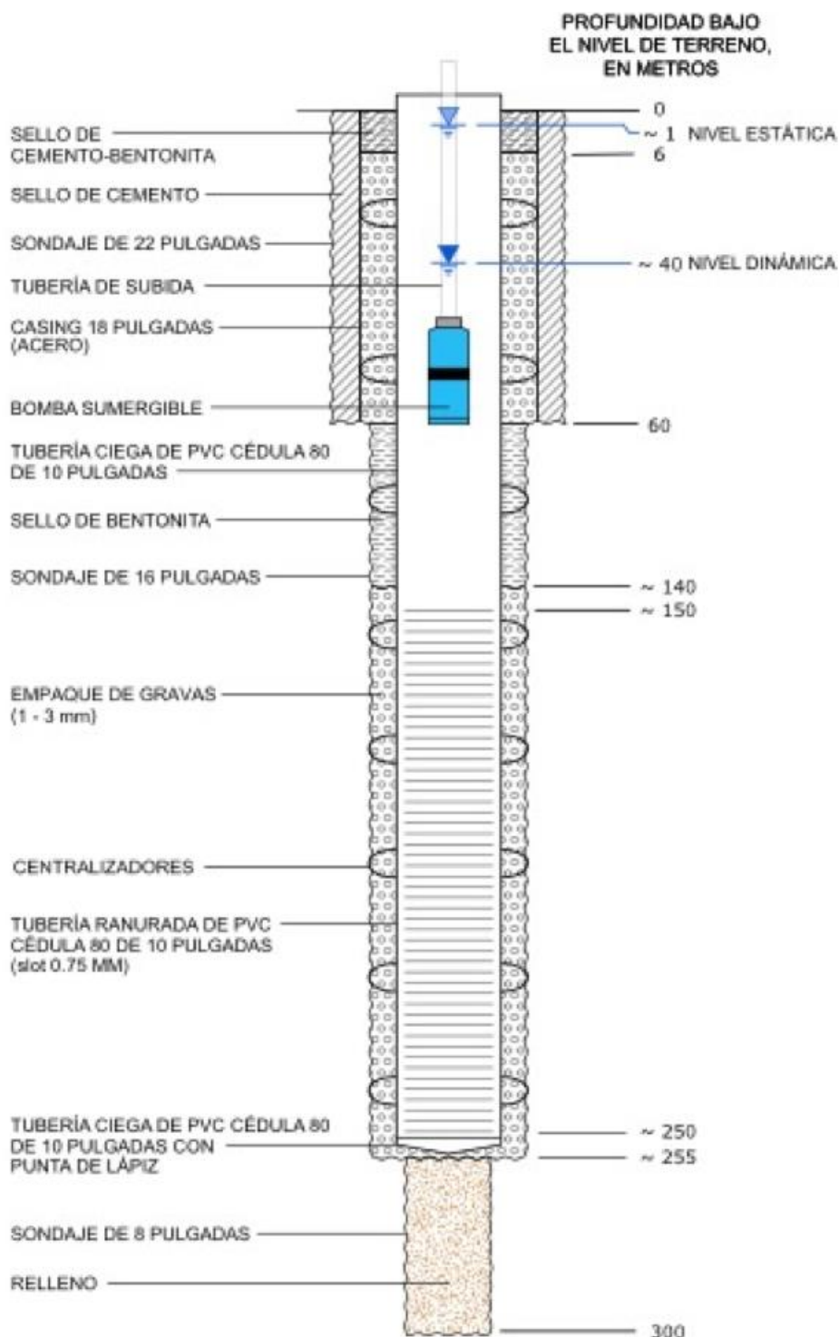
Figure 149: Construction Drawing of Production Well
