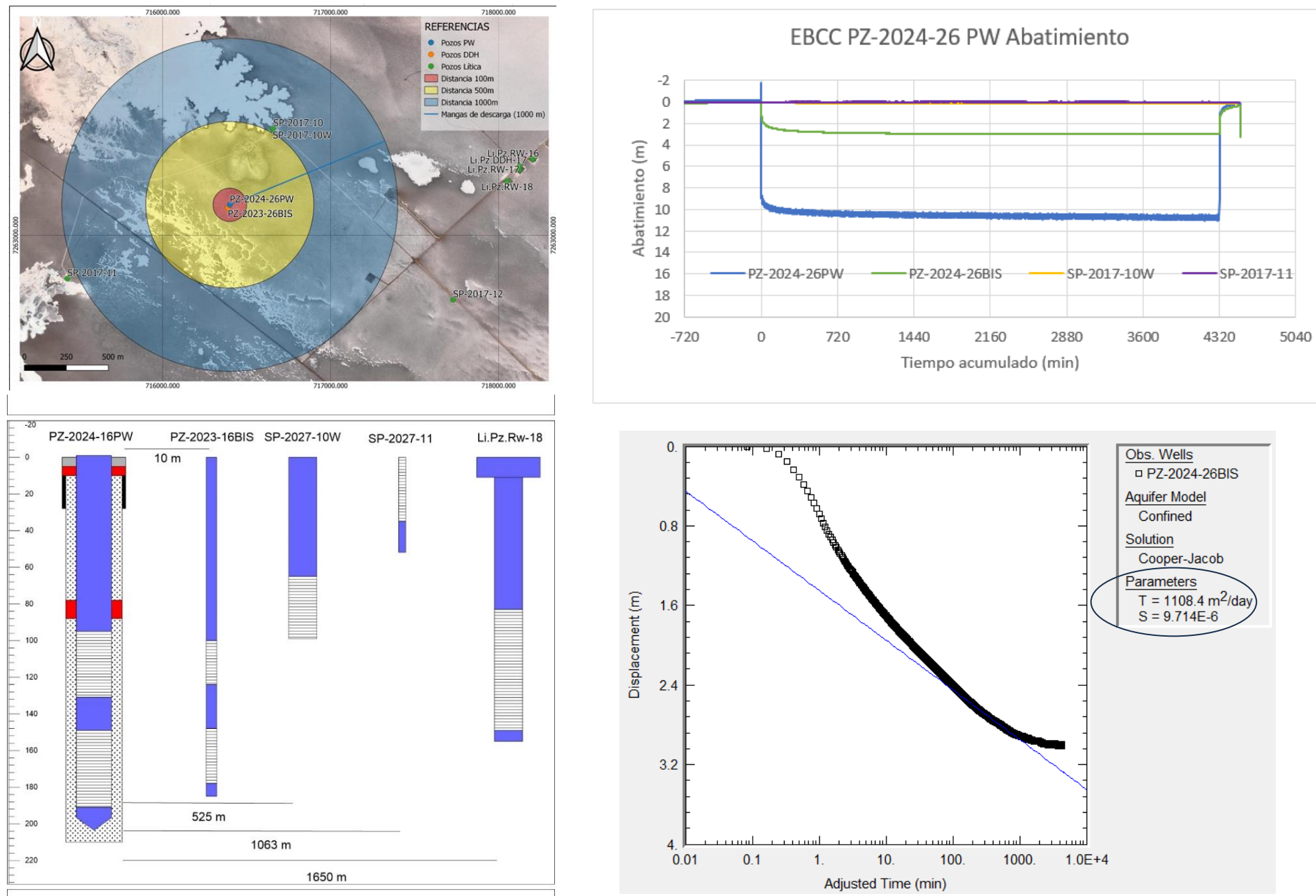
Figure 10: Location, setup and results of pumping test well PZ-2024-26
