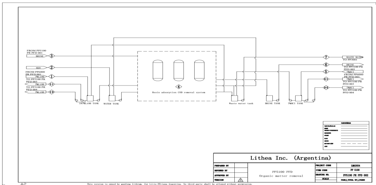
Figure 165: Flowsheet for TOC Removal Process (Source: Ganfeng, 2024)
