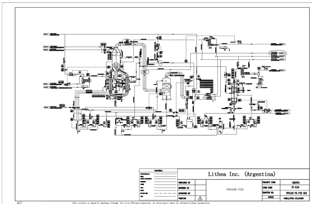
Figure 168: Flowsheet for Bipolar Membrane Electrodialysis (Source: Ganfeng, 2024)
