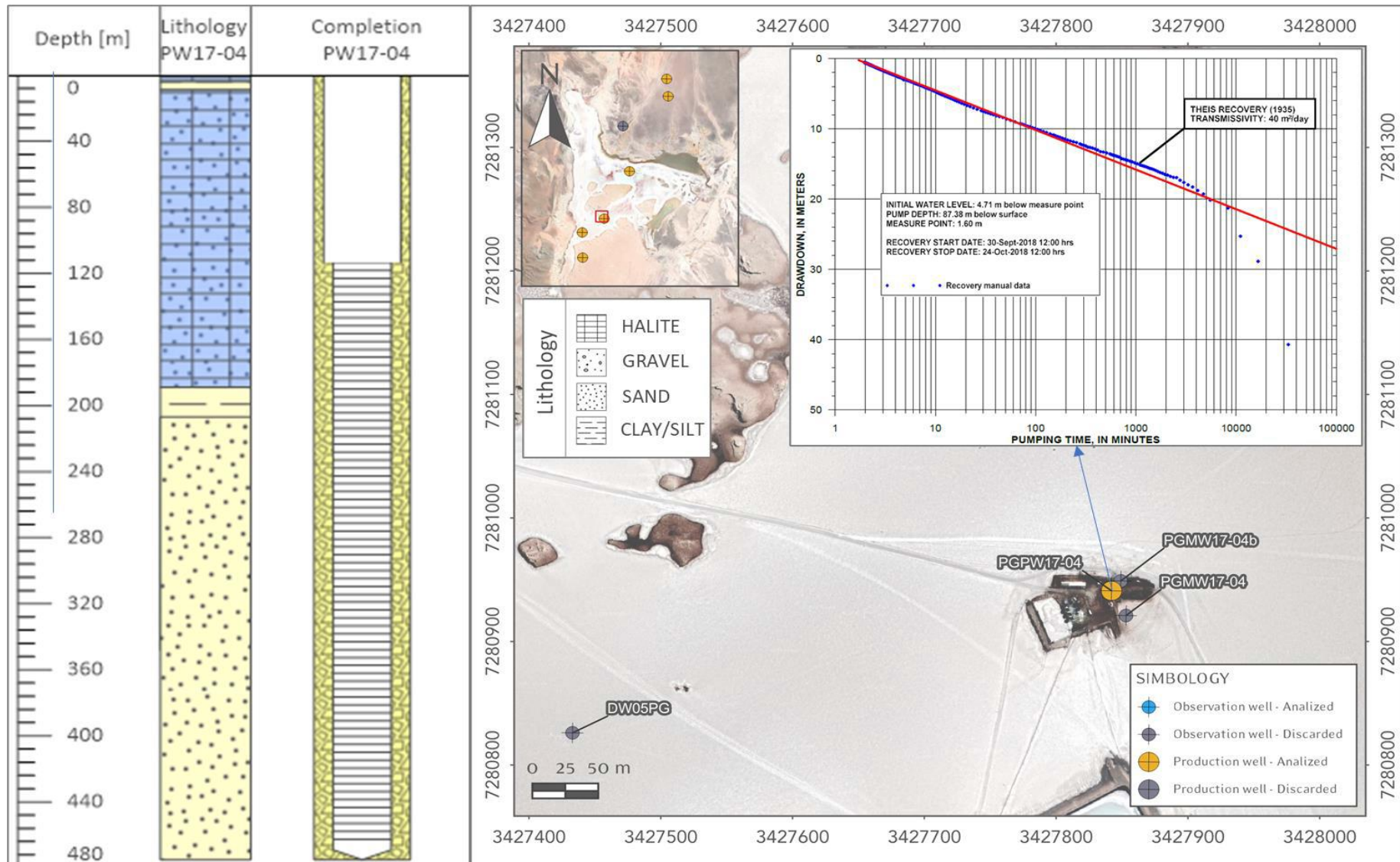
Figure 12: Location, setup and results of pumping test well PGPW17-04
