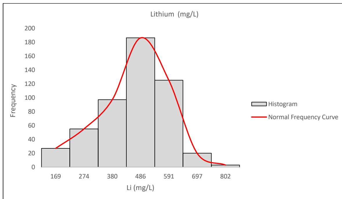
Figure 65: Histogram for Lithium Concentrations of the Complete Dataset of Samples (Source: WSP Golder, Jan 2025)
