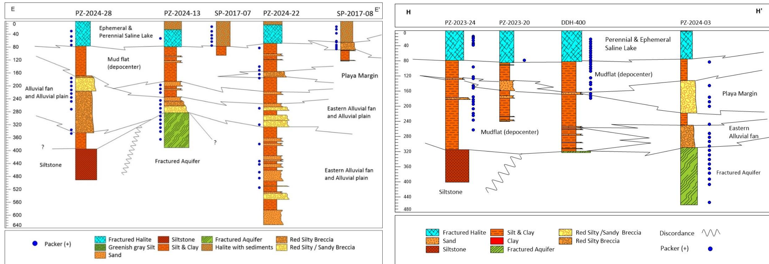
Figure 50: Cross Section E-E' (PZ-2024-28(bis), PZ-2024-13, SP-2017-07, PZ-2024-22, SP-2017-08) and Cross Section H-H' (PZ-2023-24, PZ-2023-20, DDDH-400, PZ-2024-03) (Source: WSP Golder, Jan 2025)
