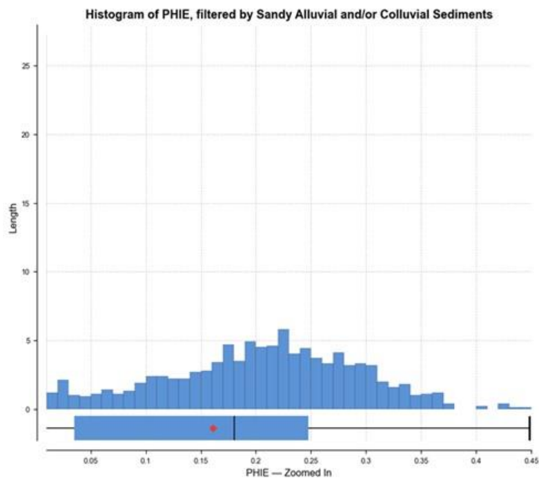
Figure 102: Histograms of the Sy (PHIEE) for the Sandy Alluvial and Colluvial Sediments (Source: WSP Golder, Jan 2025)
