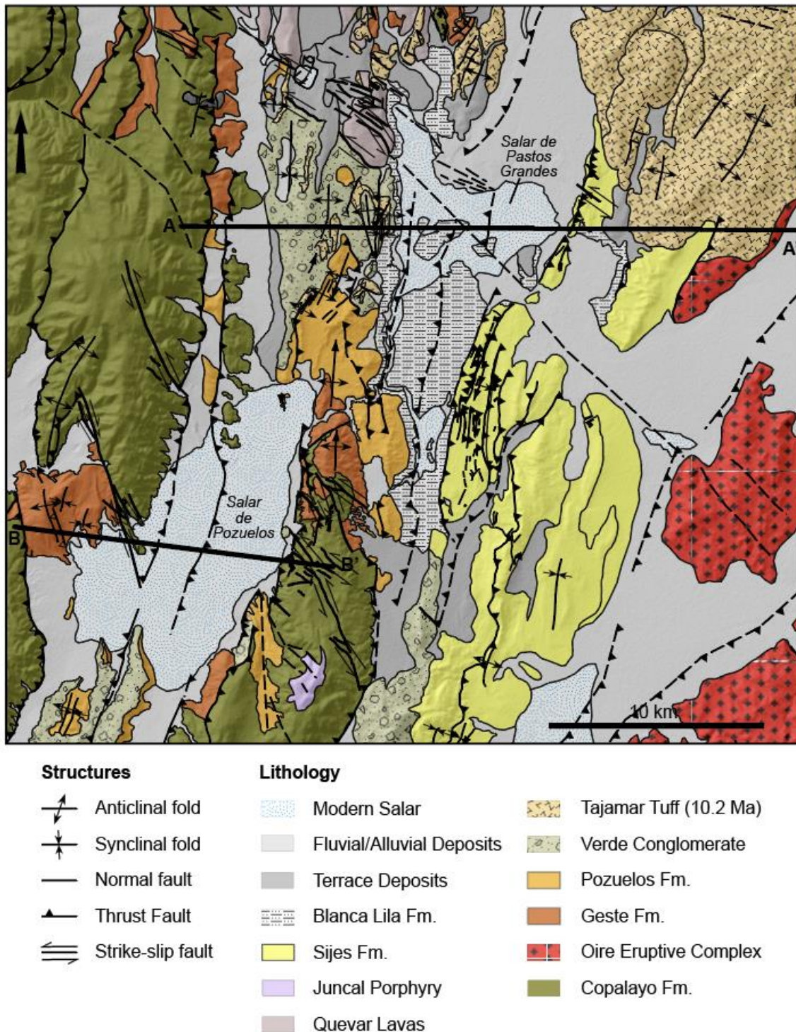
Figure 11: Geological and Structural Map of the PPG Project and Locations of Cross Section A-A' and B-B'
