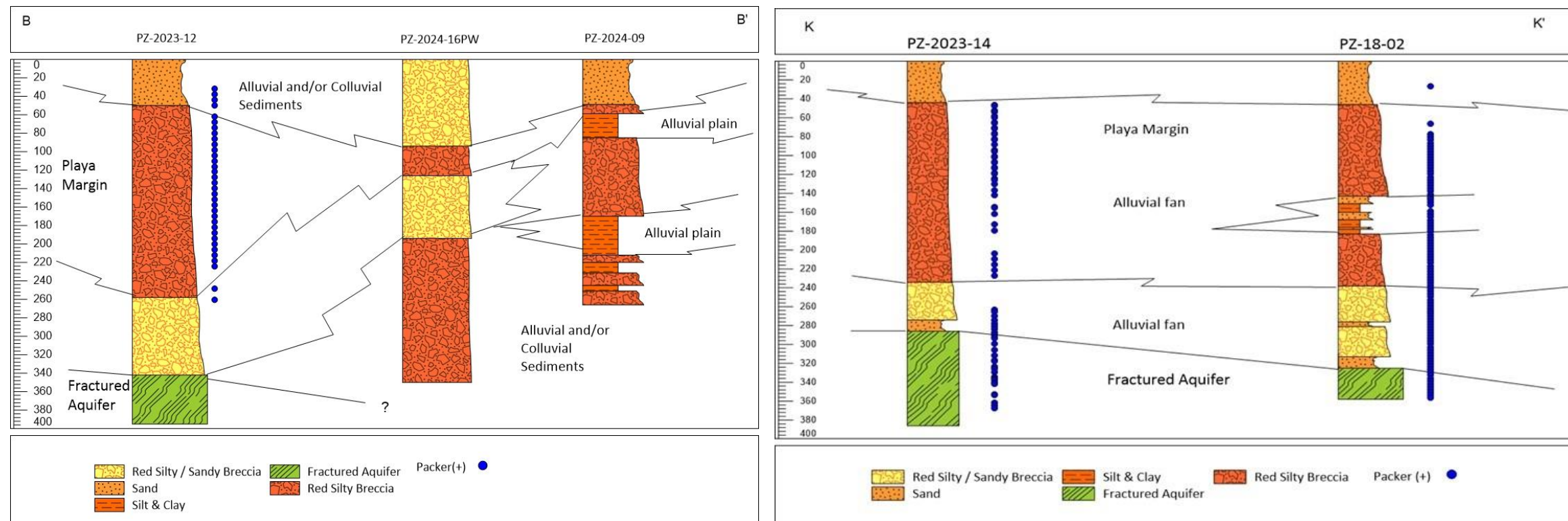
Figure 52: Cross Section B-B' (PZ-2023-12, PZ-2024-16PW, PZ-2024-09) and Cross Section K-K' (PZ-2023-14, PZ-18-02) (Source: WSP Golder, Jan 2025)
