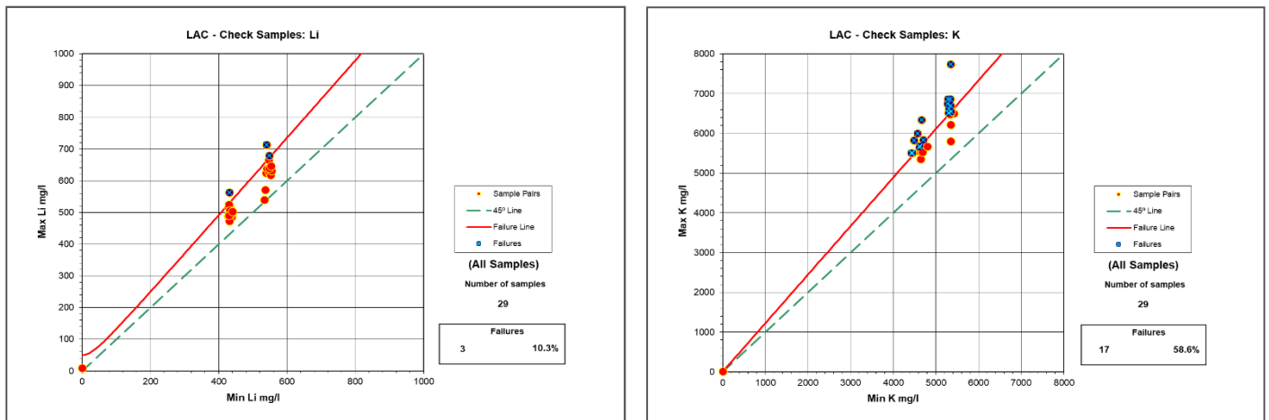
Figure 78: Max-min Plot for Li (left) and K (right) in Check Samples: ASANOVA – SGS (Source: AW, Dec 2024)
