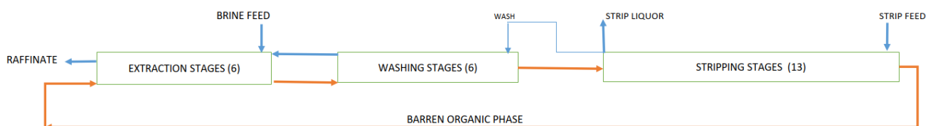
Figure 93: Process Flowsheet for Continuous Extraction Process (Source: Ganfeng, 2024)
