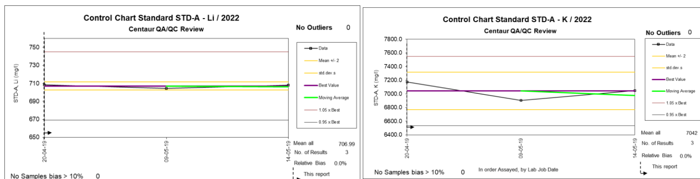
Figure 90: Max-min Plot for Lithium (left) and Potassium (right) in Duplicates – ASANO (Source: AW, Dec 2024)
