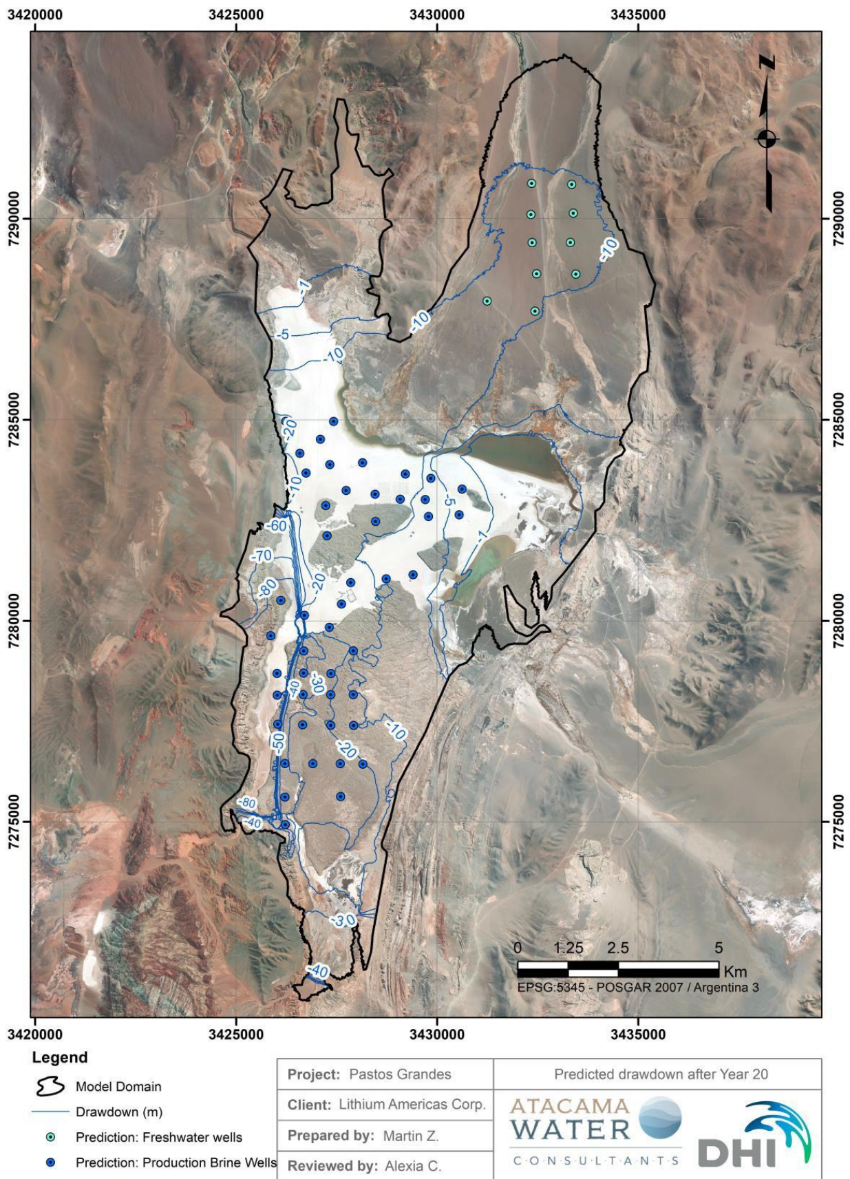
Figure 144: Predicted Drawdown after Year 20 (Source: AW, Dec 2024)
