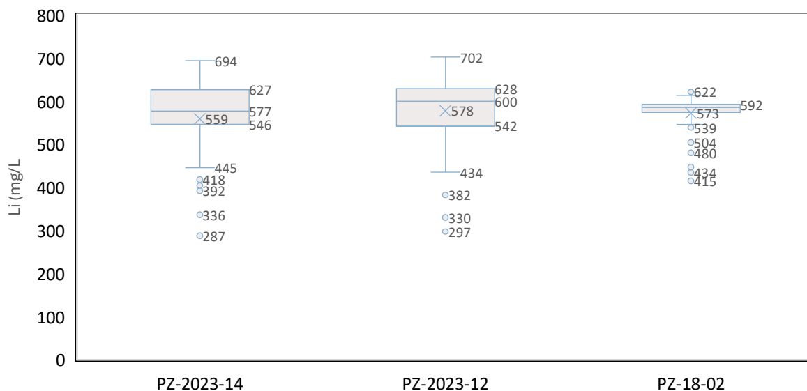
Figure 57: Lithium Concentrations in Northern Drillholes (Source: WSP Golder, Jan 2025)
