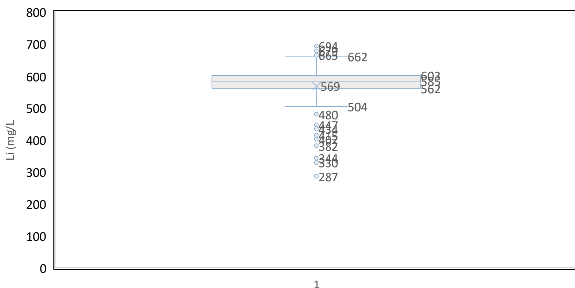
Figure 58: Lithium Concentration in the Northern Zone from Pozuelos (Source: WSP Golder, Jan 2025)
