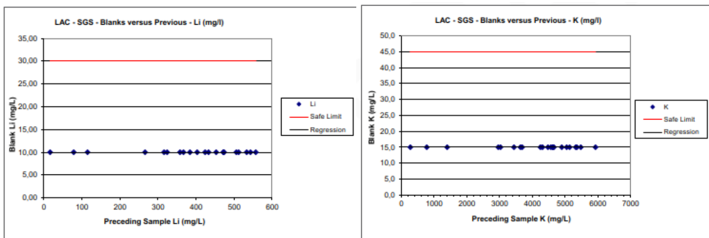
Figure 80: Blank vs Previous Samples for Lithium and Potassium – SGS (Source: AW, Dec 2024)
