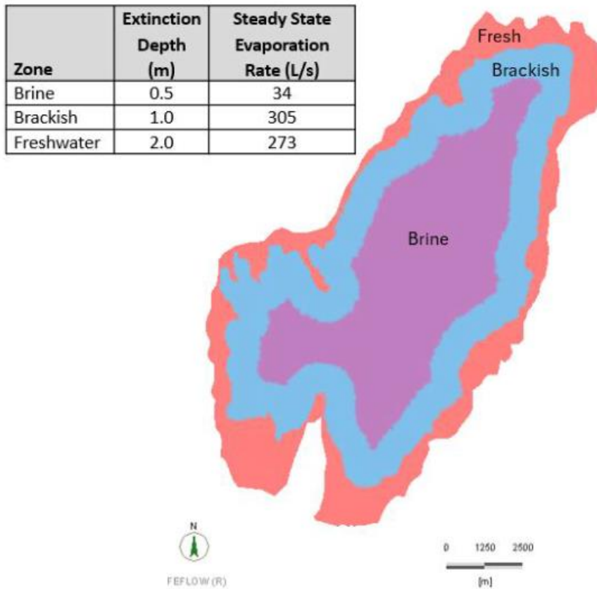
Figure 119: Evaporation Function (Source: AW, September 2024)
