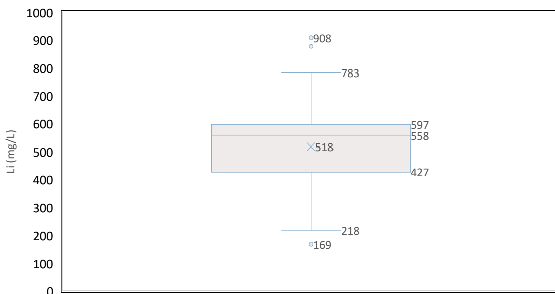
Figure 56: Lithium Concentrations from all the Exploration Samples (Source: WSP Golder, Jan 2025)
