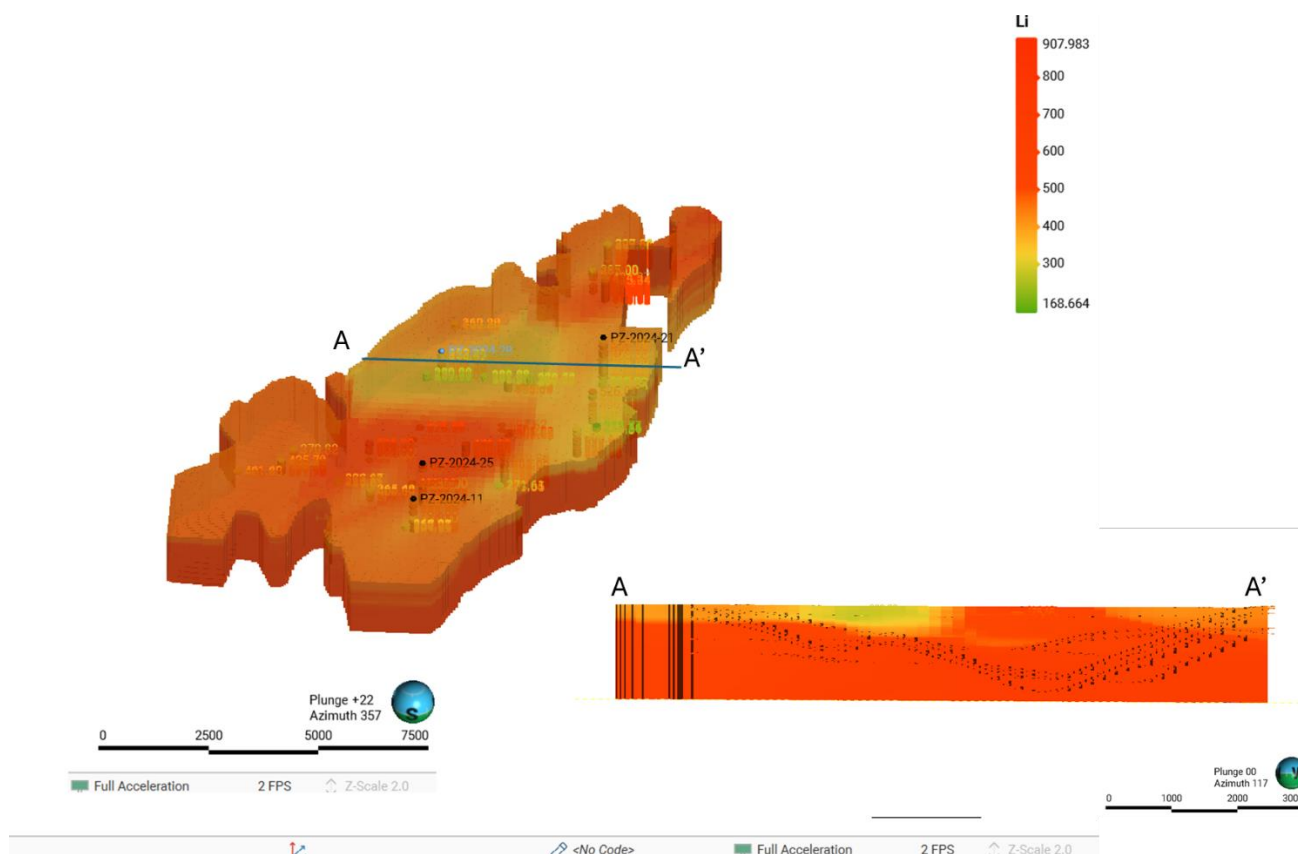
Figure 105: Lithium Distribution from the Block Model (Source: WSP Golder, Jan 2025)
