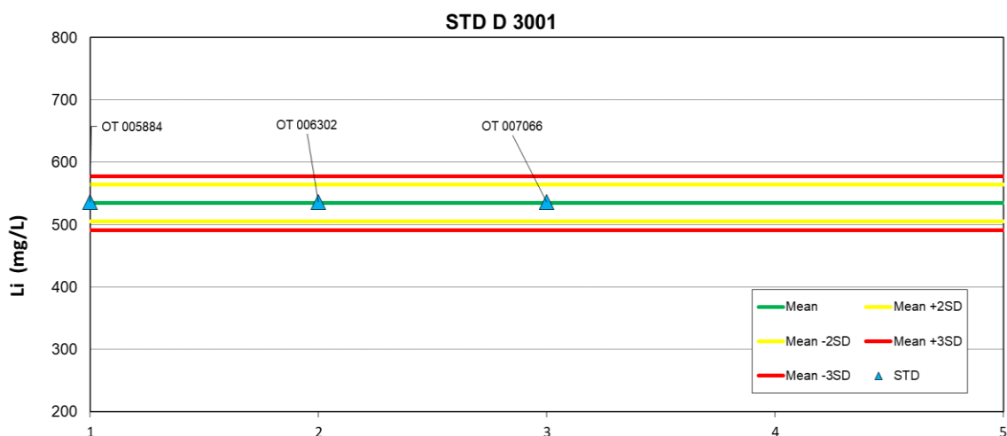
Figure 71: Performance of the Reference Sample TDS D 3001 (Source: WSP Golder, Jan 2025)
