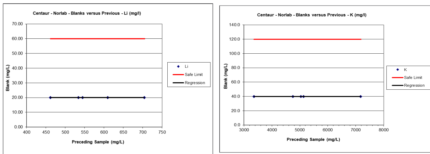
Figure 89: Blank vs Previous Samples for Lithium (left) and Potassium (right) – ASANO (Source: AW, Dec 2024)
