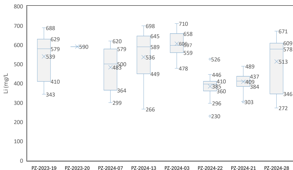
Figure 60: Lithium Concentrations from the Central Drillholes (2023-2024 Exploration) (Source: WSP Golder, Jan 2025)
