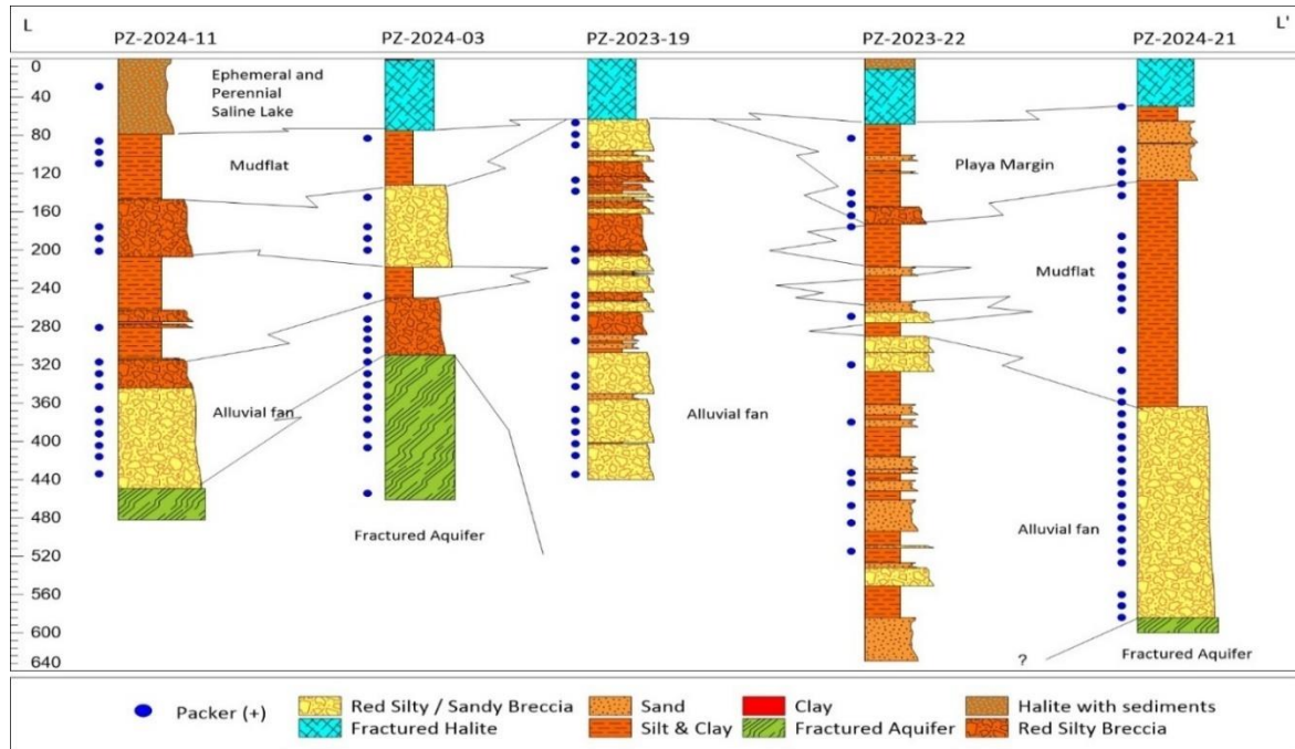
Figure 48: South-North Cross- Section L-L' PZ-2024-11, PZ-2024-03, PZ-2023-19, PZ-2023-22, PZ-2024-21 (Source: WSP Golder, Jan 2025)
