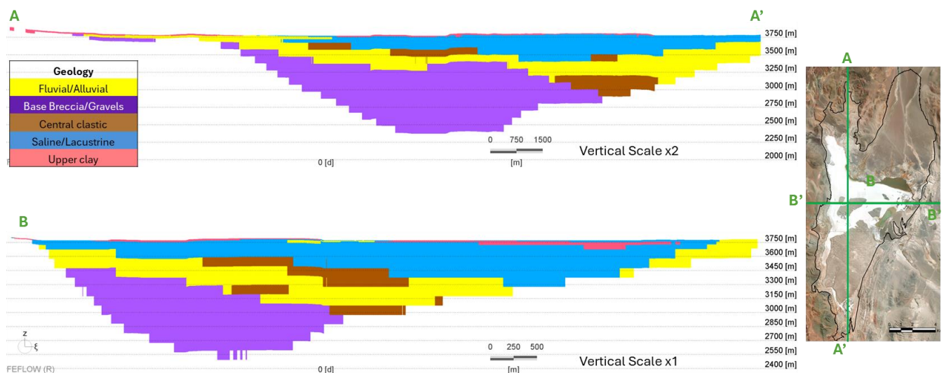
Figure 136: Hydrogeological Units in Cross Sections (Source: AW, Dec 2024)
