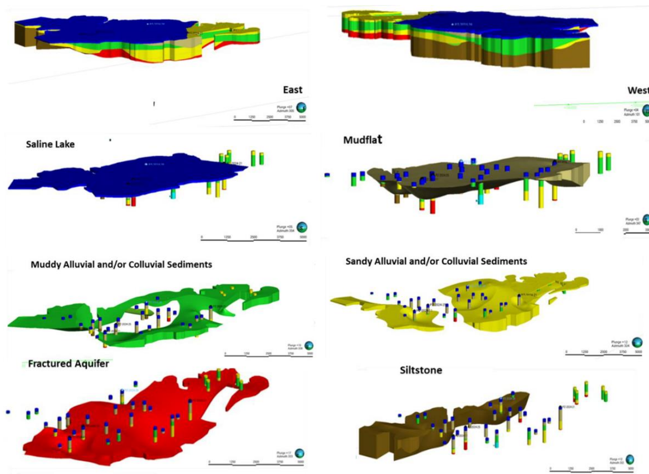
Figure 99: Hydrostratigraphic Units from the Hydrostratigraphic Model (Source: WSP Golder, Jan 2025)
