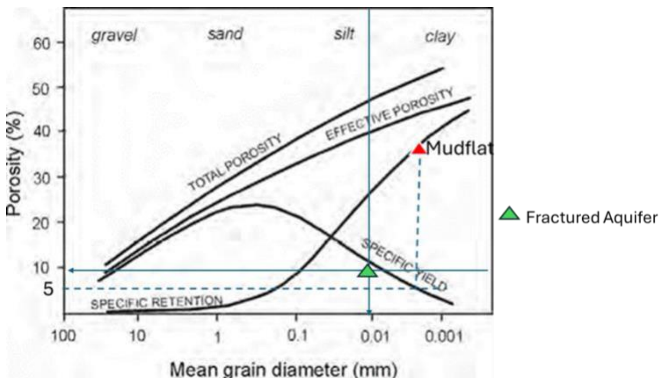
Figure 103: Porosity relationships for unconsolidated material (Source: Johnson 1967)
