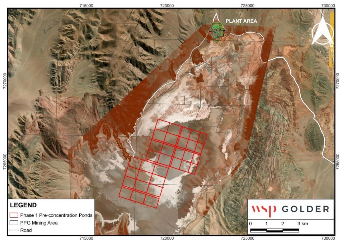
Figure 152: Phase 1 Ponds Layout
