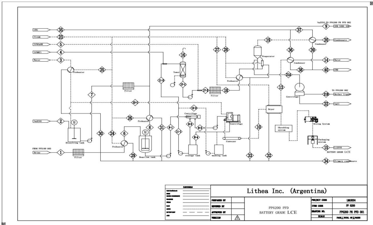
Figure 169: Flowsheet for Lithium Carbonate Plant (Source: Ganfeng, 2024)
