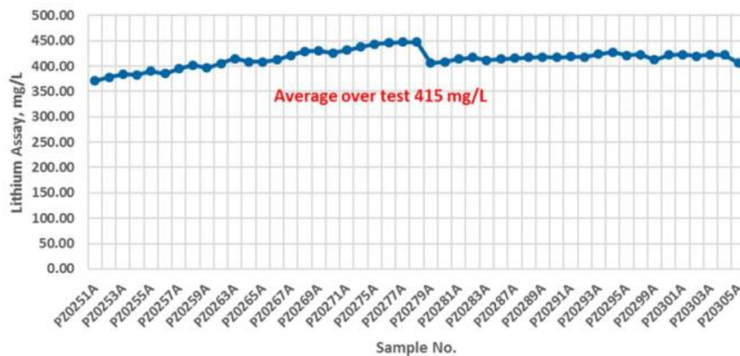
Lithium Assay During WPZ-18-01 Continuous Pumping Test
