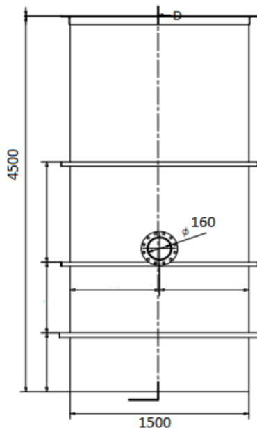
Figure 208: Pumping Well Details (Source: Ganfeng, 2024)
