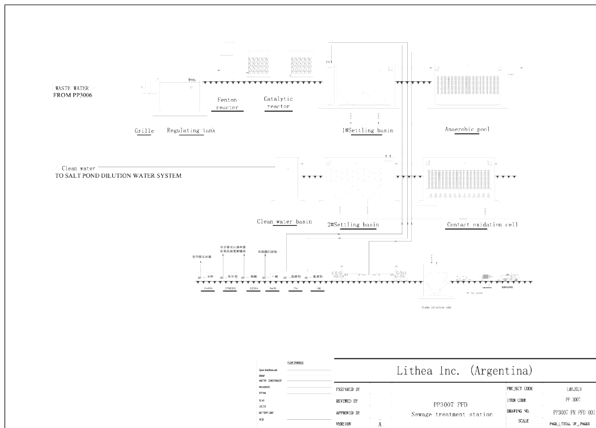
Figure 160: Process Flow Diagram of Sewage Treatment Station (Source: Ganfeng, 2024)
