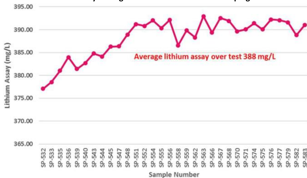
Lithium Assay During SP-2017-2W Continuous Pumping Test
