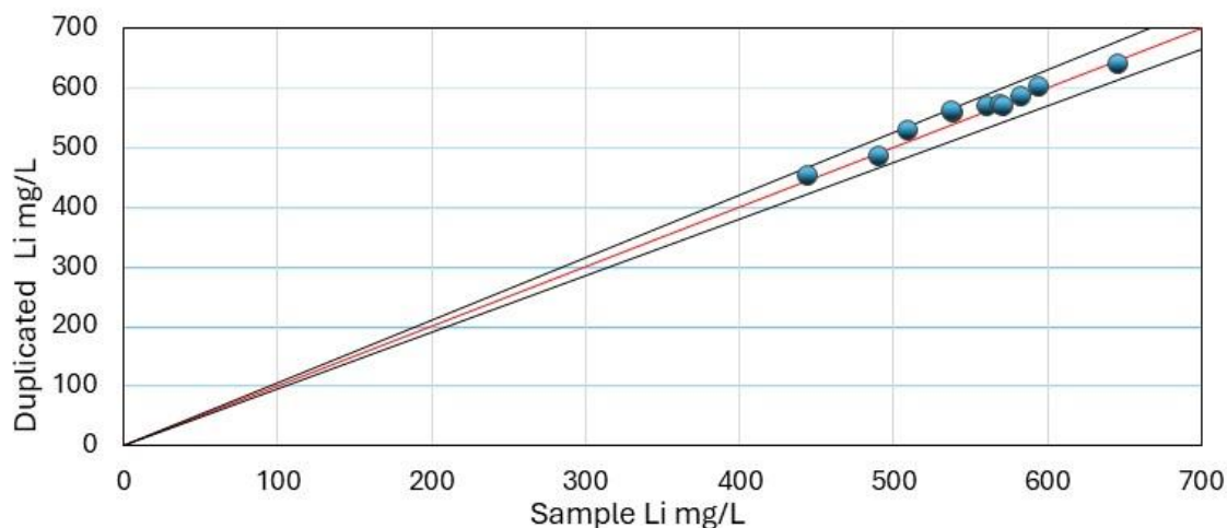
Figure 73: Duplicate Vs Original Samples (Source: WSP Golder, Jan 2025)
