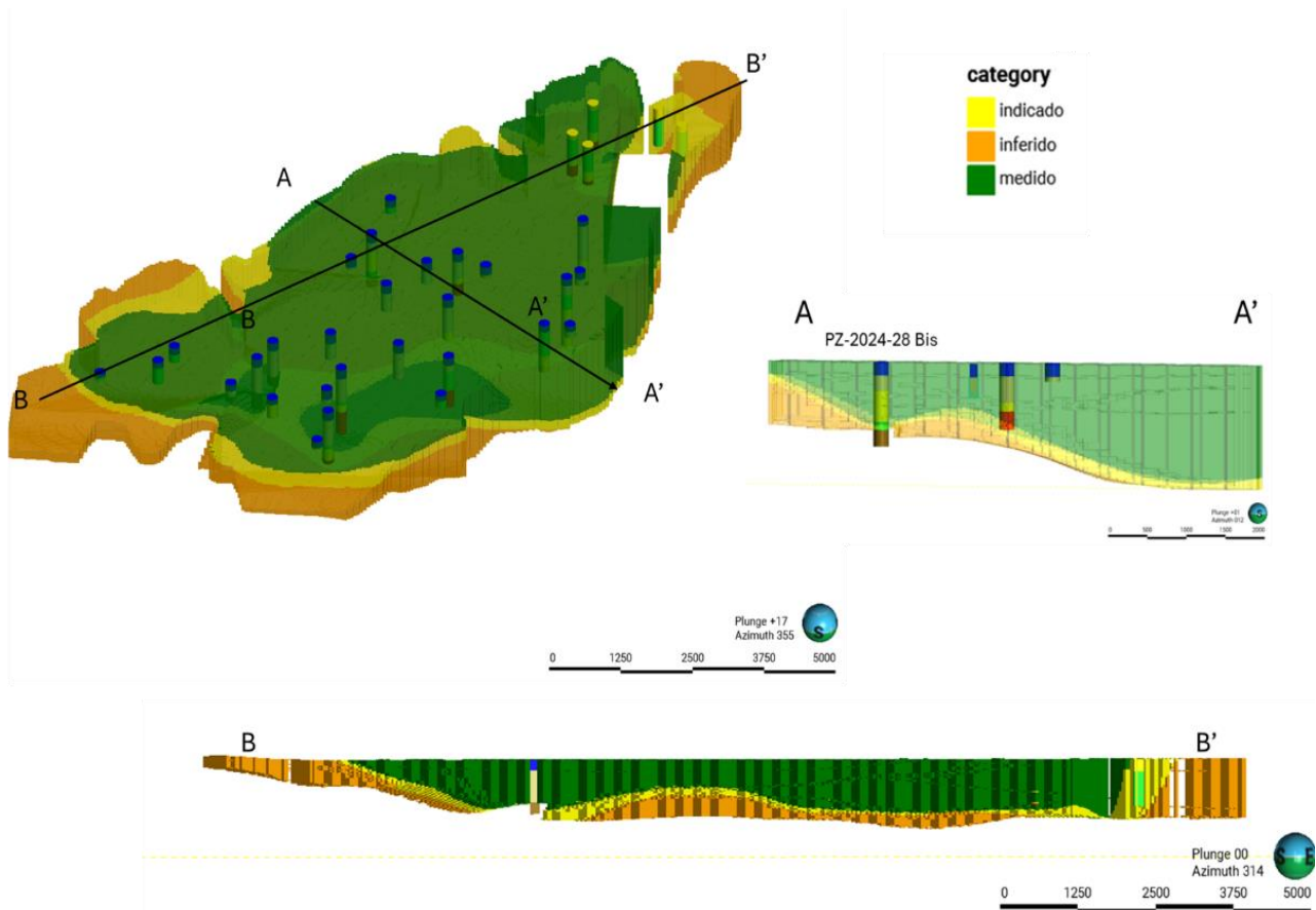
Figure 106: Measured, Indicated and Inferred Resource Distribution (Source: WSP Golder, Jan 2025)
