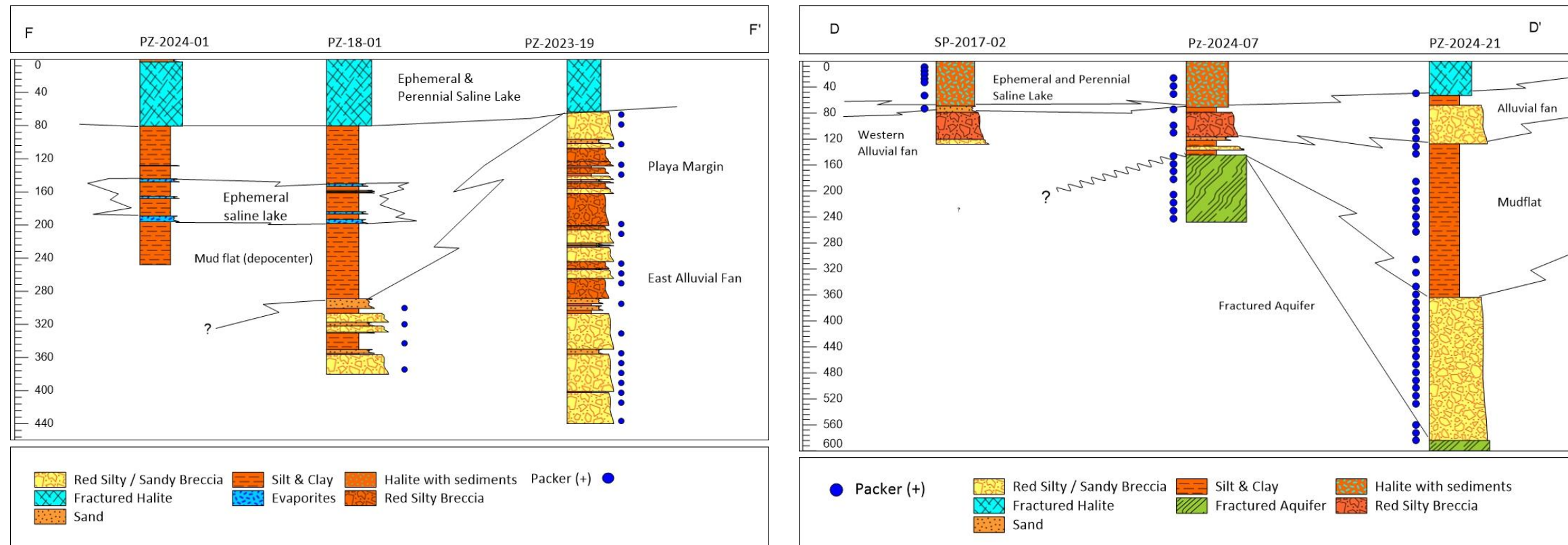
Figure 51: Cross Section F-F' (PZ-2024-01, PZ-118-01, PZ-2023-19) and Cross Section D-D' (SP-2017-02, PZ-2024-07, PZ-2024-21) (Source: WSP Golder, Jan 2025)
