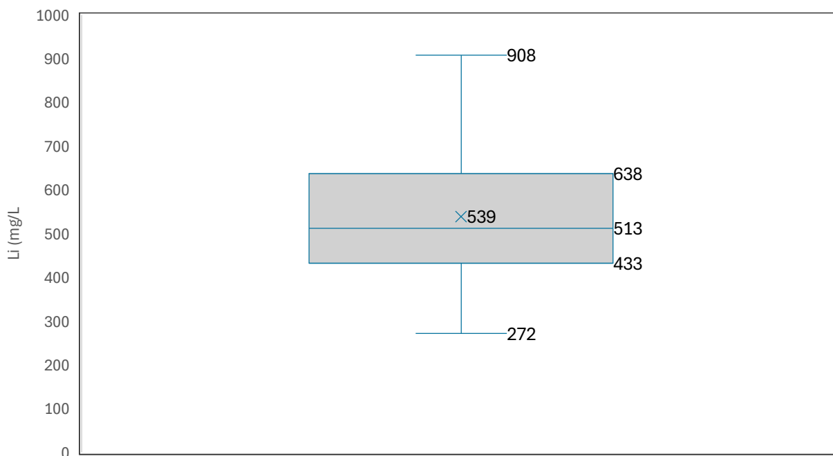
Figure 64: Lithium Concentrations from the Southern Zone from Pozuelos (Source: WSP Golder, Jan 2025)
