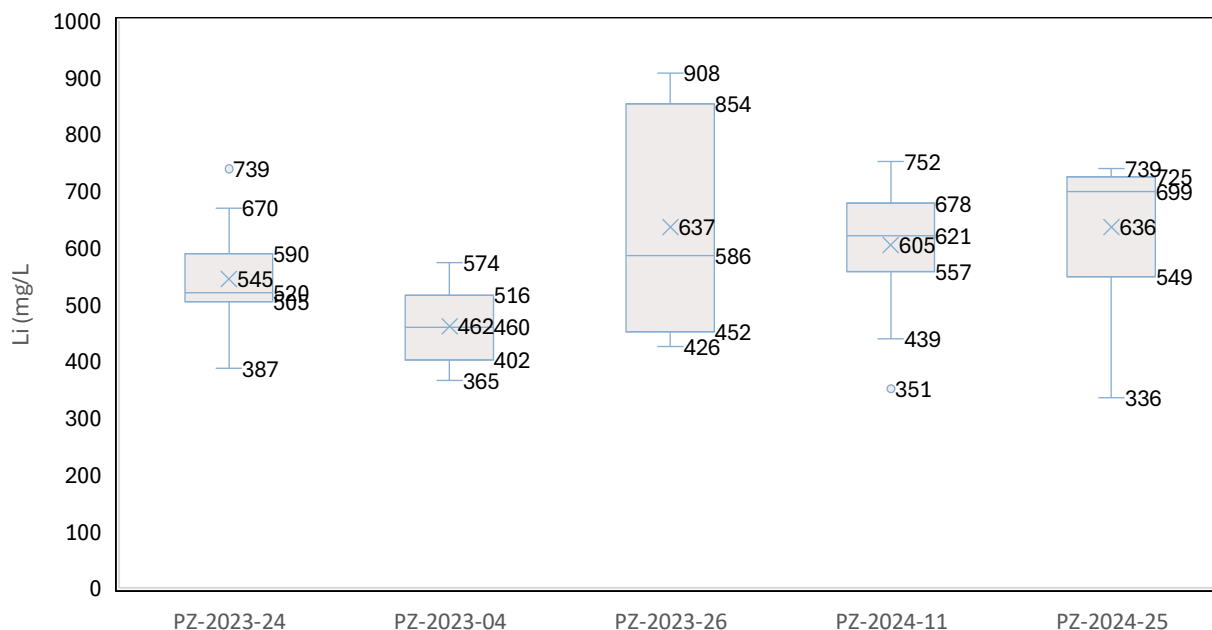
Figure 63: Lithium Concentrations from the Southern Drillholes (2023-2024 Exploration) (Source: WSP Golder, Jan 2025)
