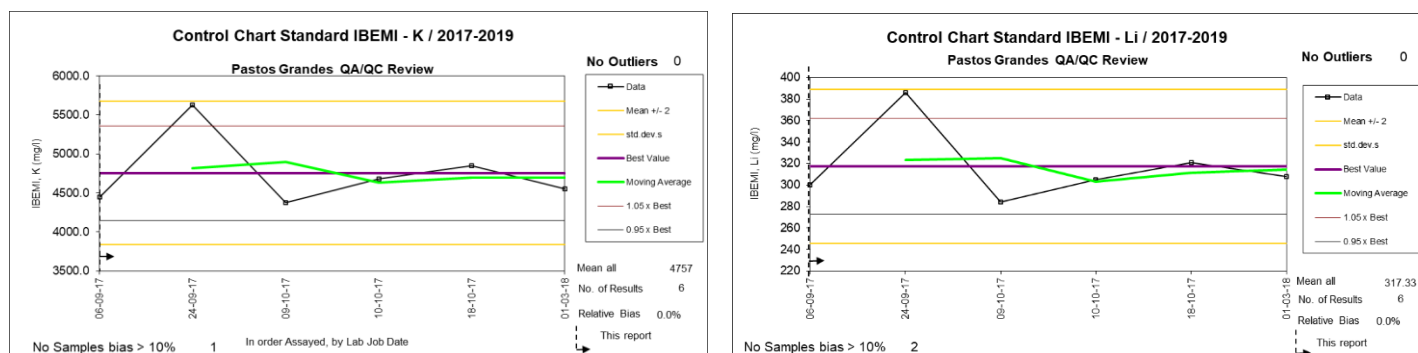
Figure 83: Graphical Analysis of Li (top) and K (bottom) within 'INBEMI' Standards Assayed by SGS (Source: AW, Dec 2024)
