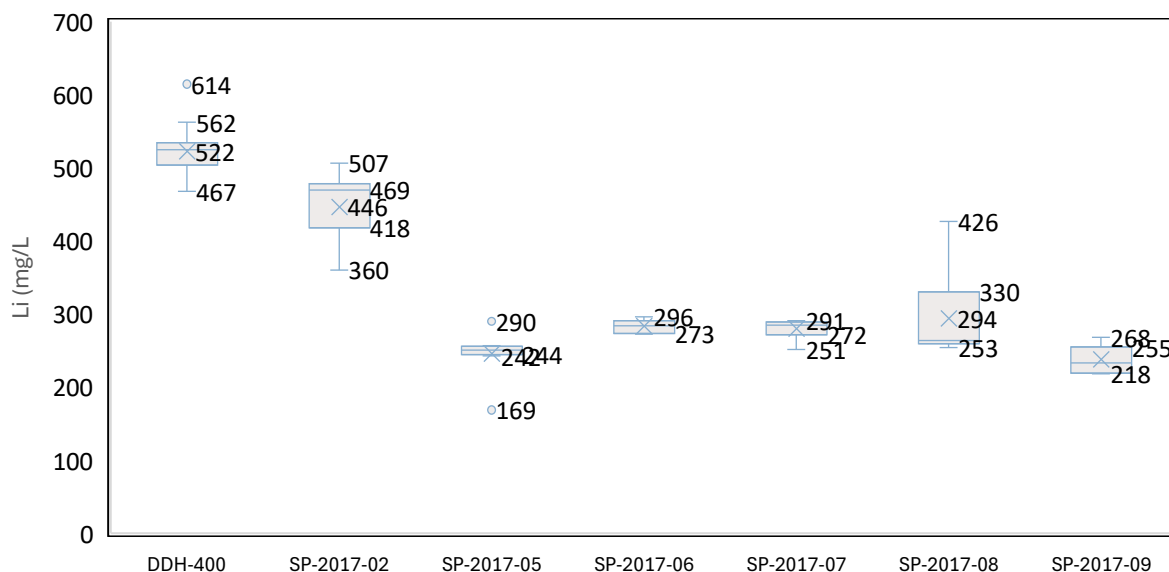
Figure 59: Lithium Concentrations Central Drillholes (2017-2018 exploration) (Source: WSP Golder, Jan 2025)
