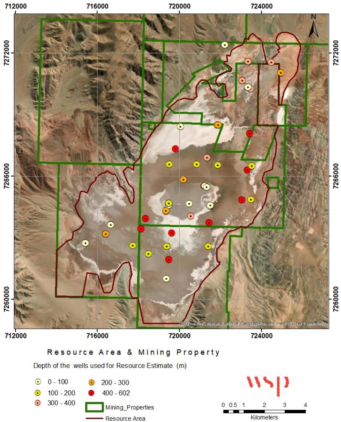
Figure 98: Resource Area vs Mining Properties (Source: WSP Golder, Jan 2025)
