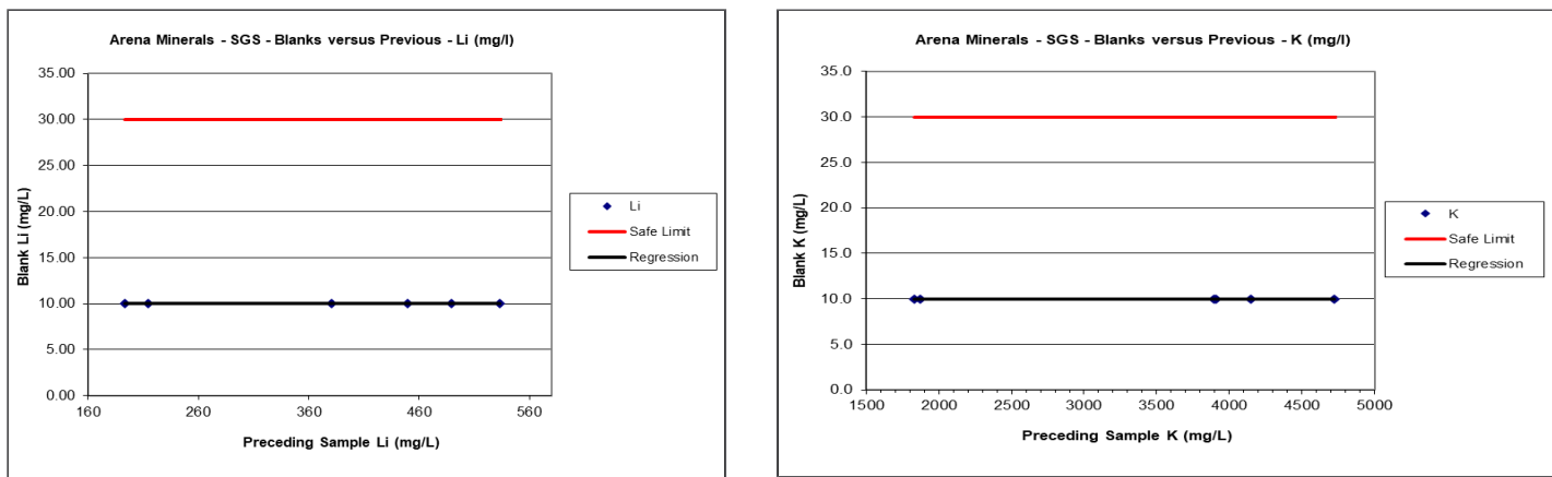
Figure 85: Blank vs Previous Samples for Lithium (left) and Potassium (right) – SGS (Source: AW, Dec 2024)
