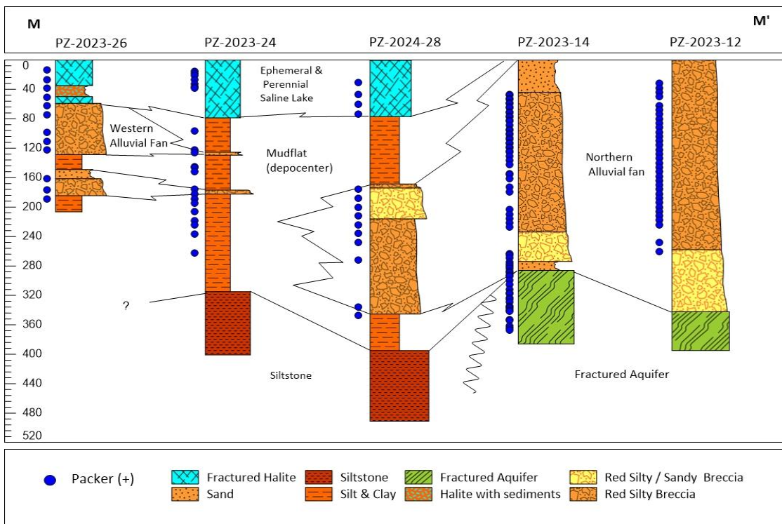
Figure 47: South-North Cross Section M-M' PZ-2023-26, PZ-2023-24, PZ-2024-28(bis), PZ-2023-14, PZ-2023-12 (Source: WSP Golder, Jan 2025)
