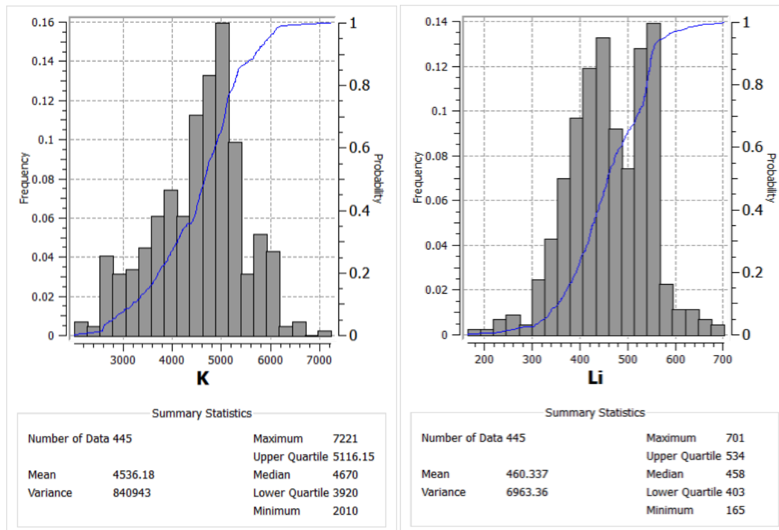
Figure 113: Lithium and Potassium Histograms and Cumulative Distributions for Region I (Source: AW, Dec 2024)
